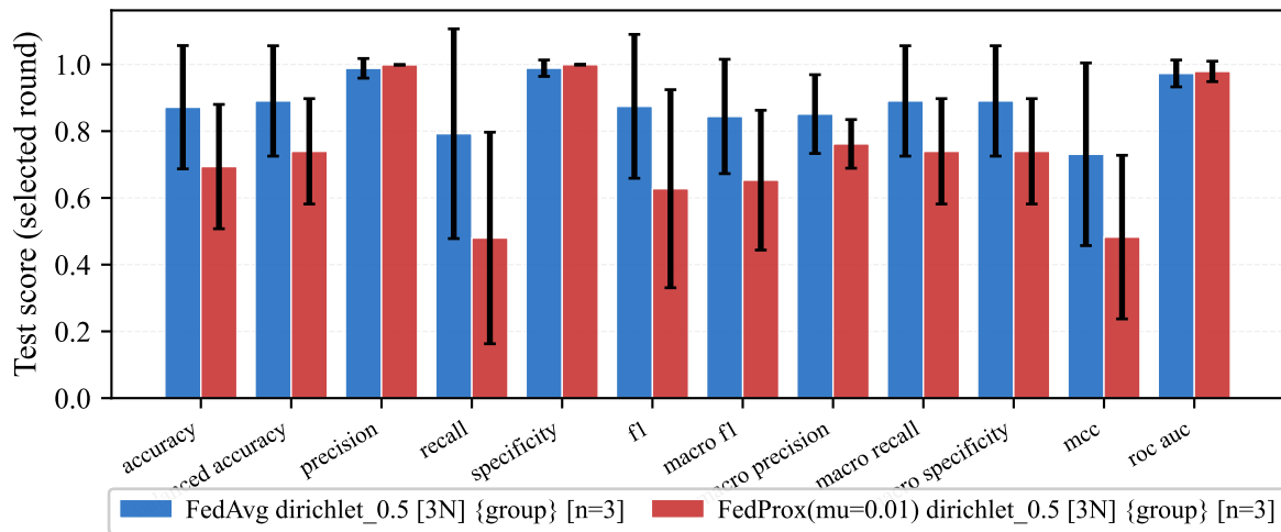
Selected-round test metrics — dirichlet_0.5
