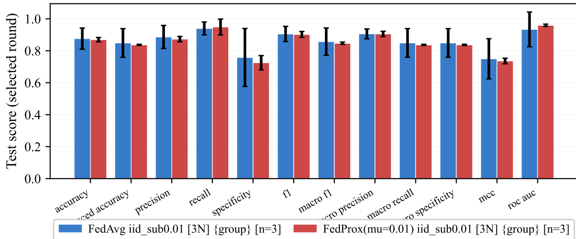
Selected-round test metrics — iid_sub0.01
