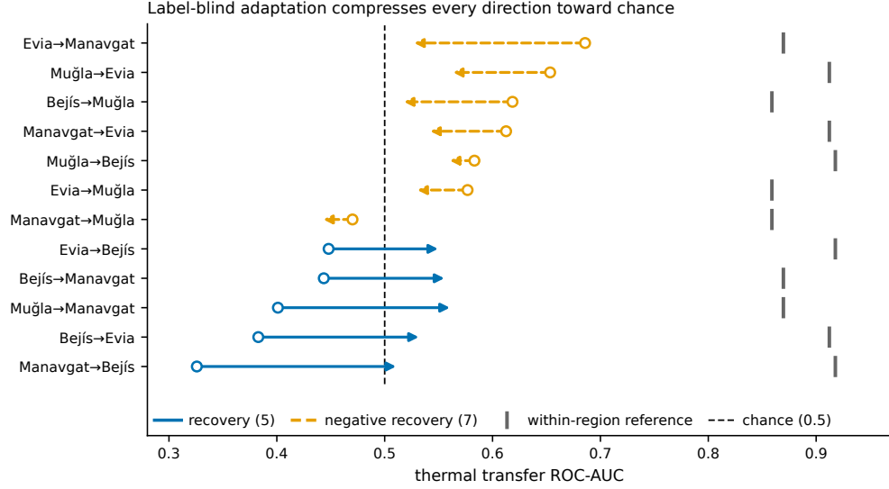
Figure A.5: Label-blind adaptation regresses transfer onto the level a model reaches on an unseen scar, rather than recovering it. All 12 ordered directions among the four regions carrying the full decomposition (Manavgat, Bejís, Muğla, Evia), natural-vegetation primary population. Each row is one direction. The open circle is raw transfer ROC-AUC and the arrow runs to the best label-blind adapted result for that direction (region-wise z-score or CORAL, whichever is better); the grey vertical tick is the within-region reference for that target, and the dashed vertical rule is chance. Solid blue arrows are the five directions where adaptation moves transfer toward the within-region reference (recovery); dashed orange arrows are the seven where it moves away from it (negative recovery). Line style and colour both encode this class, because the two hues differ by only 2.30:1 in relative luminance and would nearly merge in greyscale. The pattern is the point: all six directions starting above chance are pushed down, and five of the six starting below chance are pushed up, so adaptation acts on the spread rather than on skill. The exception is Manavgat→Muğla, which starts below chance at 0.470 and is pushed further down to 0.443. The worst case is Evia→Manavgat, where raw transfer of 0.686 is dragged down to 0.527 against a within-region reference of 0.870, a recovered fraction of -0.862 . No arrow reaches its within-region tick.
