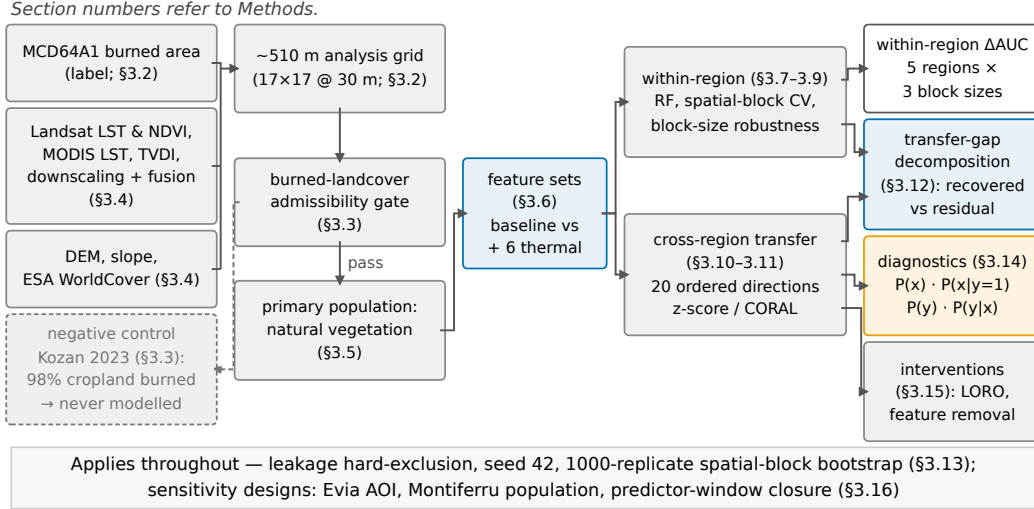
Figure C.1: Processing pipeline and evaluation programme. Flow from source products (left) to the transfer and diagnostic programme (right); every box carries the Methods subsection that specifies it. The five source products (MCD64A1 burned area, Landsat Collection 2 Level-2, MOD11A1, Copernicus DEM GLO-30 and ESA WorldCover) merge onto the reconstructed \sim 510 m analysis grid ( 17 \times 17 pixels of the 30 m reference grid). The burned-landcover admissibility gate has two outcomes: regions that pass proceed to the natural-vegetation primary population, while the rejecting branch (grey, dashed) terminates in the Kozan 2023 negative control, whose burned area is 98% cropland and which is never modelled. The dashed connector deliberately carries no arrowhead onward, so the control cannot be read as entering the pipeline. Feature sets feed two evaluations in parallel: within-region (random forest under spatial-block cross-validation) and cross-region transfer (source-only, 20 ordered directions, with label-blind z-score and CORAL adaptation). Their levels are combined in the transfer-gap decomposition (§3.12). The footer states what applies throughout: leakage hard-exclusion, seed 42, 1000-replicate spatial-block bootstrap (§3.13), and the sensitivity designs (§3.16). Section references are verified against the Methods heading list when the figure is built.
