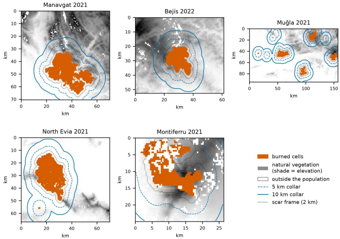
Figure S1. The five study areas at cell level. Grey shading is the elevation of the natural-vegetation cells, white cells lie outside this population, and burned cells are orange. The dashed and solid blue lines are the 5 km and 10 km distance collars, and the dotted black lines the 2 km scar frames of Table 2 (Section 3.12). In Muğla one burned area reaches the eastern edge of the study area (15 burned cells on the edge), so its collars are cut there. Axes give approximate distances in km on the ~500 m grid. Drawn by paper/figures/figS1_study_areas.py from the released modelling datasets.
