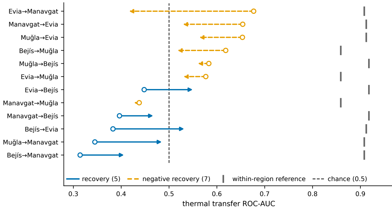
Label-blind adaptation compresses the matrix toward chance
