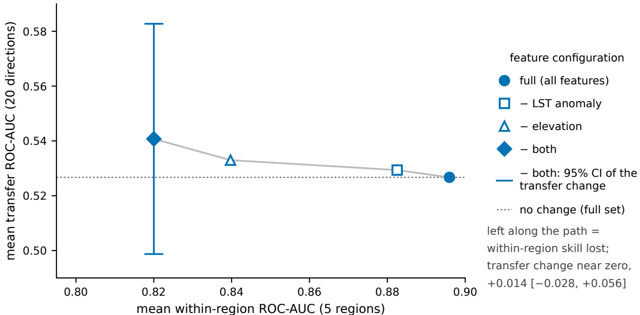
Feature removal costs within-region skill; the transfer change is near zero
