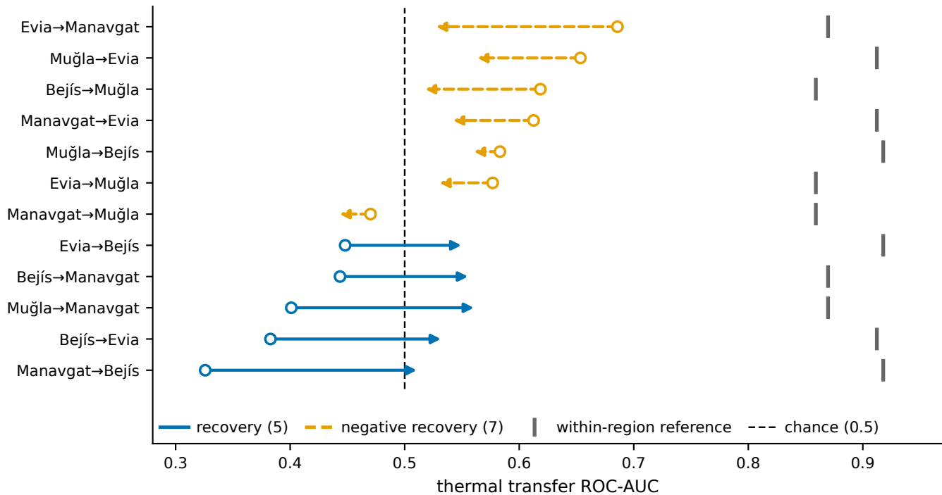
Label-blind adaptation compresses every direction toward chance
