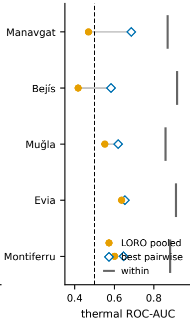
(b) Pooling never beats the best single source
