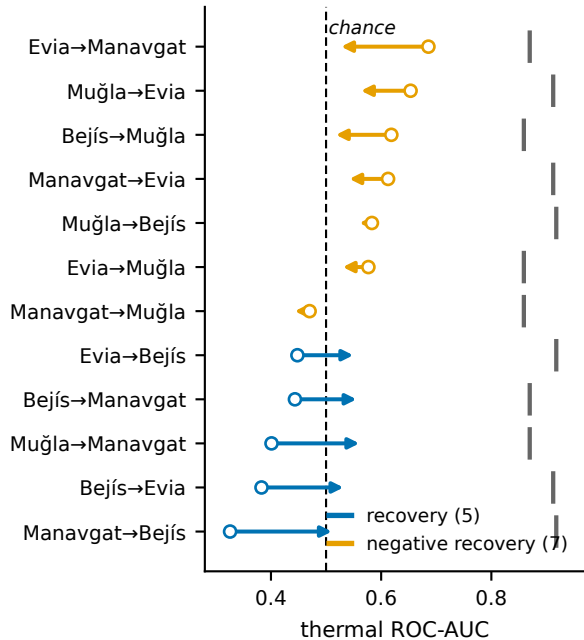
(a) Adaptation compresses toward chance raw ○ → best adapted; grey | = within
