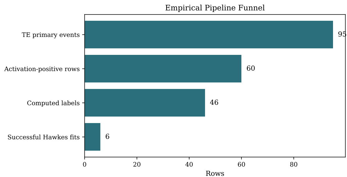
Figure 1: Empirical pipeline funnel from primary macro candidates through successful Hawkes fits.
