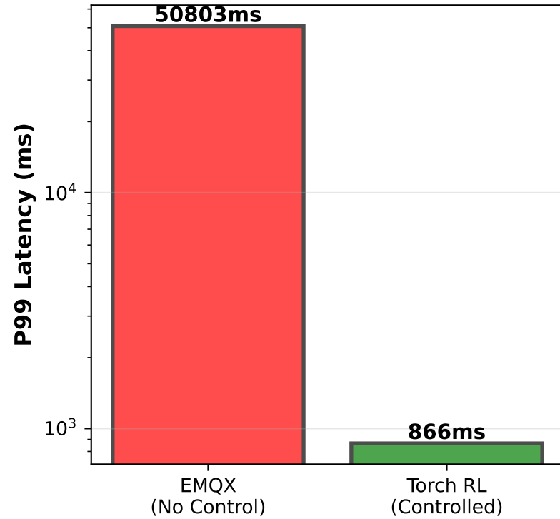
P99: RL Control Reduces by 98.3%
