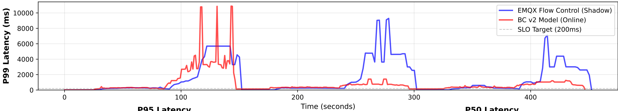
P99 Latency Over Time - Dynamic Network Scenario
