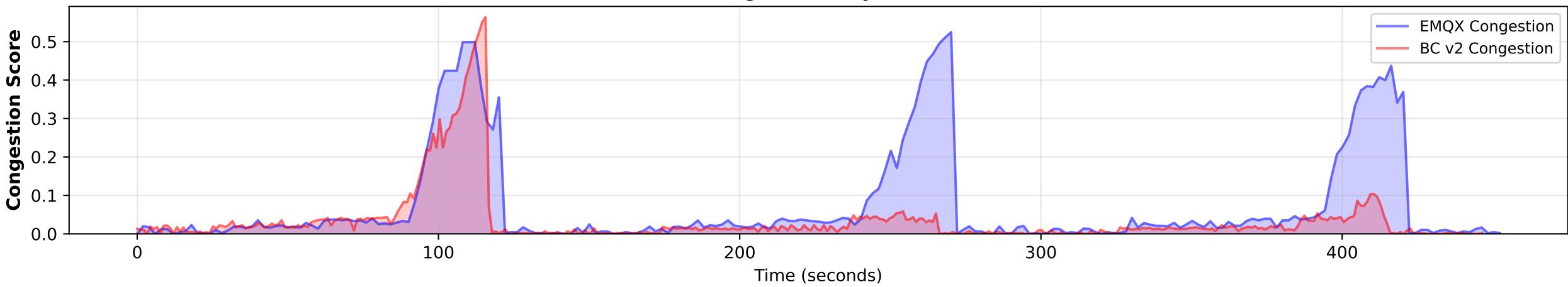
Network Congestion (Dynamic Phases)
