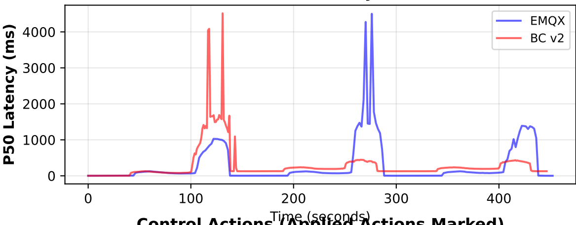
P50 Latency
