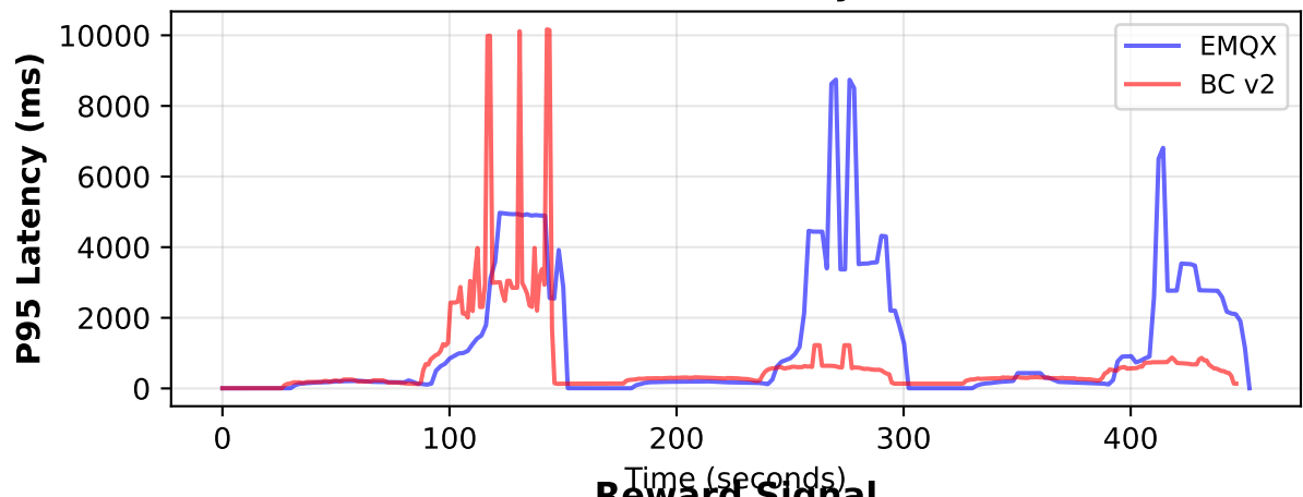
P95 Latency
