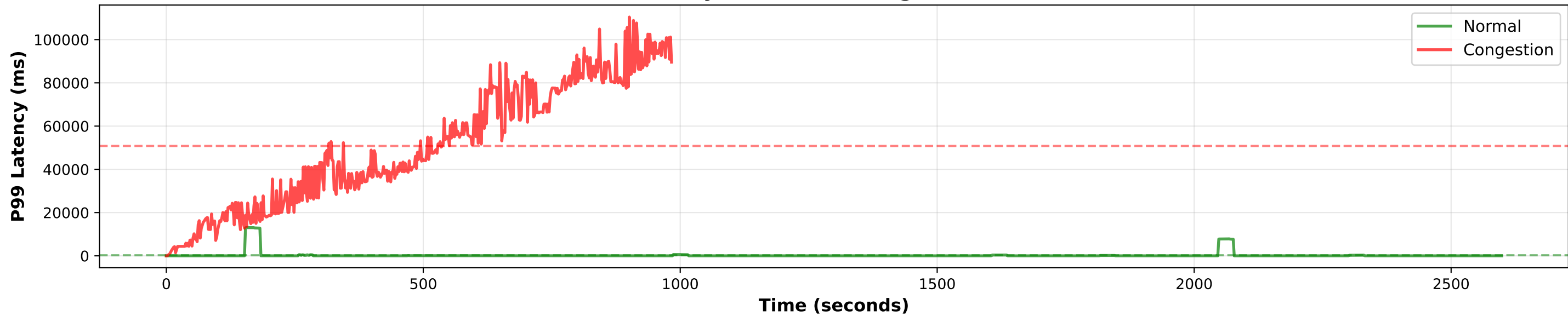
P99 Latency: Normal vs Congestion Scenario
