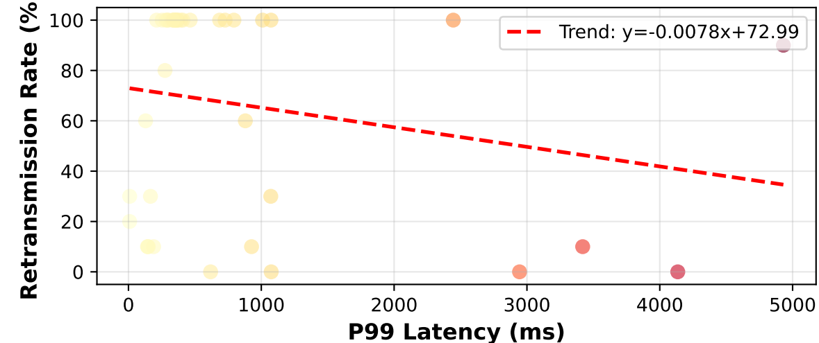
P99 vs Retransmission ( r=-0.126 )
