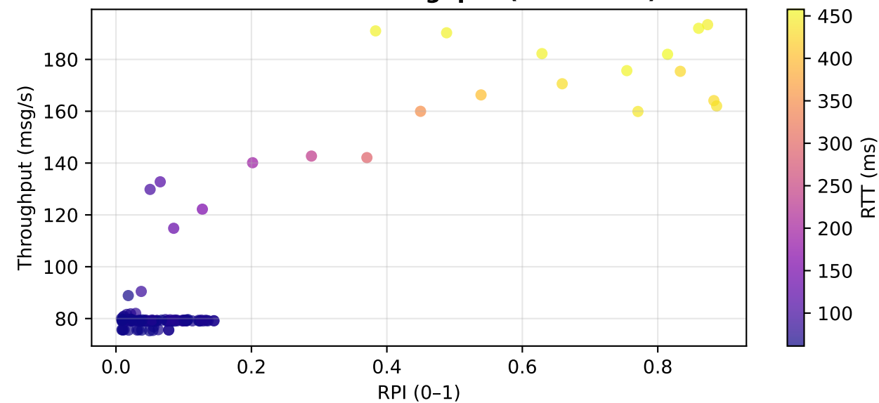
Torch: RPI vs Throughput (color=RTT)
