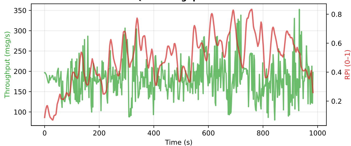
EMQX: Throughput & RPI
