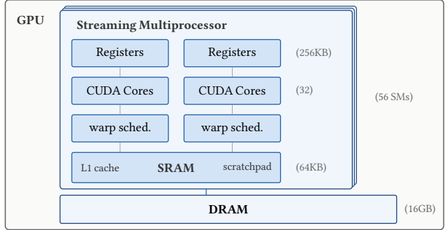
Fig. 2. Simplified SIMT hardware organization, annotated with NVIDIA Pascal P100 capacities. A GPU contains many streaming multiprocessors (SMs); each SM has two warp schedulers, two groups of CUDA Cores, a large partitioned register file, an L1 cache (SRAM), and programmer-managed shared memory (scratchpad). All SMs share the GPU’s off-chip DRAM.
