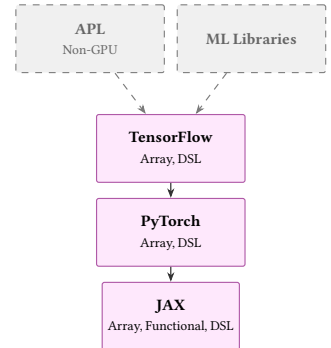
Fig. 29. Machine learning DSLs.
