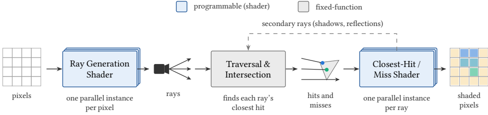
Fig. 31. A (simplified) ray-tracing pipeline, as exposed by languages like OptiX [270] and HLSL [229]. Like the rasterization pipeline in Figure 1, it consists of both programmable stages and hardware-accelerated fixed-function stages.
