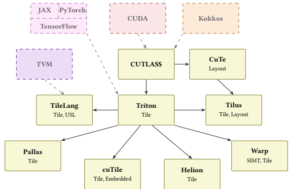
Fig. 38. Descendants of CUTLASS [334] and Triton [343].
