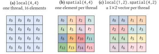
Fig. 52. Three layouts assigning the elements of a 4 \times 4 tile to threads, in the notation of Figure 51; each cell is labeled by the thread that holds it in its registers. Composition (c) yields the distributed fragments: each thread holds a small contiguous vector, and consecutive threads hold adjacent vectors.
