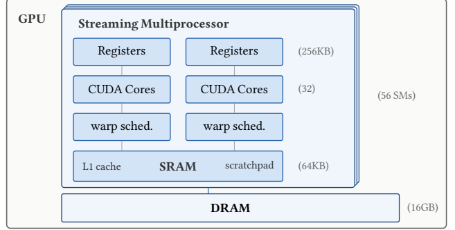
Fig. 2. Simplified SIMT hardware organization, annotated with NVIDIA Pascal P100 capacities. A GPU contains many streaming multiprocessors (SMs); each SM has two warp schedulers, two groups of CUDA Cores, a large partitioned register file, an L1 cache (SRAM), and programmer-managed shared memory (scratchpad). All SMs share the GPU’s off-chip DRAM.
