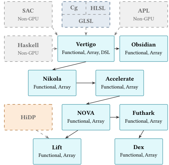
Fig. 26. Functional array languages for GPUs.
