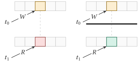
Fig. 46. The SDV semantics of GPUVerify [38]. Left: reading a pending write causes a run-time error. Right: after synchronizing, the read succeeds.
