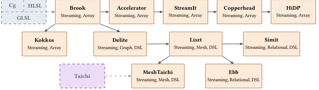
Fig. 19. Descendants of Brook [52]. Dashed boxes and lines indicate connections to or from languages outside this immediate slice of the genealogy in Figure 16.
