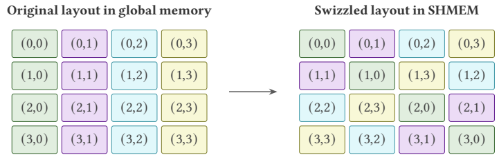
Fig. 13. A swizzle of a 4×4 tile. Labels (r,c) identify the original location of elements. The swizzle moves each entry to column c \oplus r without changing its row, where \oplus is bitwise XOR.
