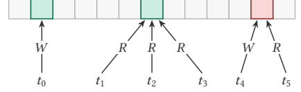
Fig. 47. VerCors [43] allows each memory location an exclusive writer or shared readers. A writer and reader at the same location conflict.
