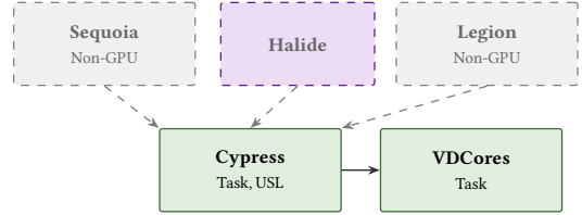
Fig. 42. Task-based languages for GPU programming.
