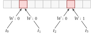
Fig. 49. In a benign data race (left), threads write the same value to the same location. In a harmful data race, threads write different values. Faial [76] cannot distinguish between the two; later work on FaialAA [213] was more precise.
