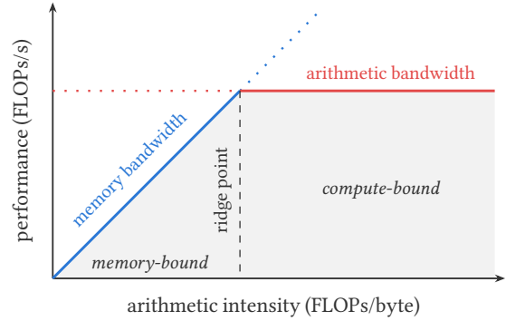
Fig. 5. The roofline model [363]. A kernel’s maximum attainable performance is capped by the lower of two ceilings.
