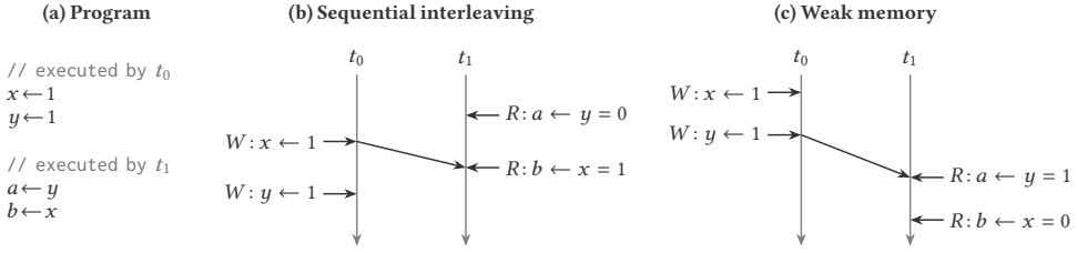
Fig. 44. In (a), a program where t_0 executes x \leftarrow 1 ; y \leftarrow 1 and t_1 executes a \leftarrow y ; b \leftarrow x . Initially x = y = 0 . In (b) and (c), two possible parallel executions of this program; diagonal arrows link writes to reads that observe them. In (b), threads are interleaved sequentially, and t_1 reads y before it is written. In (c), weak-memory behaviors cause t_1 to observe the write to y but not the write to x , an outcome no sequential interleaving can produce.
