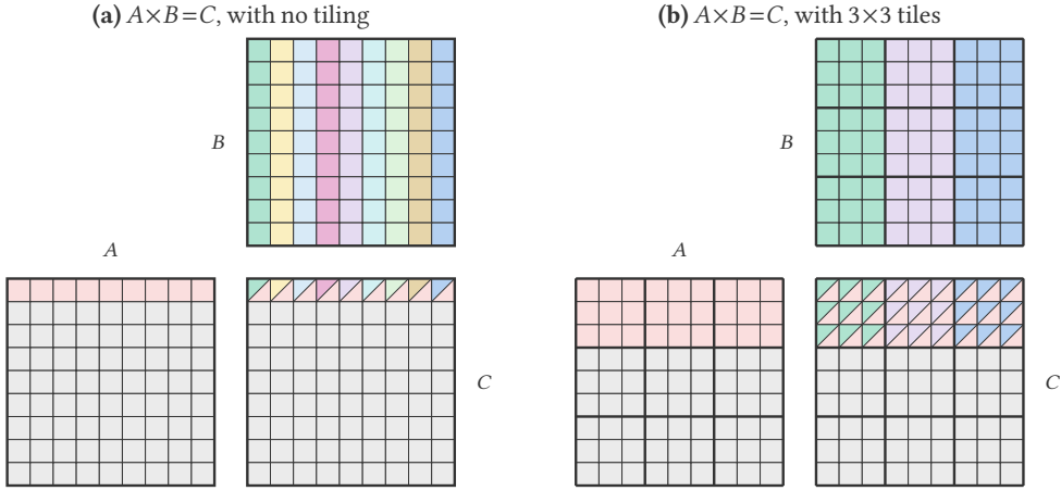
Fig. 15. Two approaches to matrix multiplication. In (a), threads compute C one scalar cell at a time; each cell is the sum of products of a cell-row of A and a cell-column of B . In (b), warps cooperate to compute C a tile at a time using Tensor Cores; one tile of C is the sum of products of a tile-row of A and a tile-column of B .
