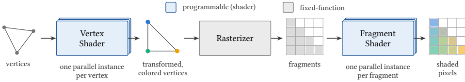
Fig. 1. A simplified graphics pipeline of the early programmable-shader era. A programmable vertex shader transforms each vertex and assigns it a color; a fixed-function rasterizer converts a triangle into the fragments it covers; and a programmable fragment shader computes each pixel’s final color from the interpolated vertex colors. Every vertex and fragment is processed independently, so each shader stage is inherently data-parallel.
