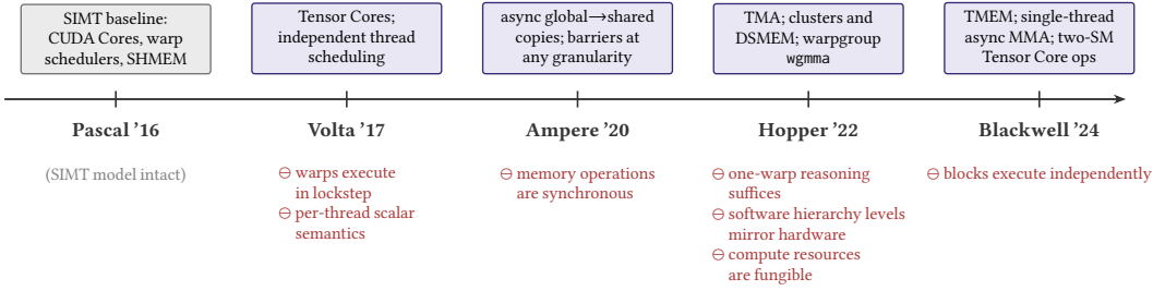
Fig. 14. Five generations of NVIDIA microarchitectures. Above the timeline: the major hardware capabilities each generation introduced. Below: the SIMT assumptions that those capabilities removed.
