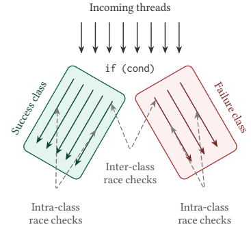
Fig. 45. Parametric flows handling a conditional in GKLEE p [207]. Races are checked between pairs of arbitrary threads within the classes that succeed and fail the conditional and between representatives of the two classes.
