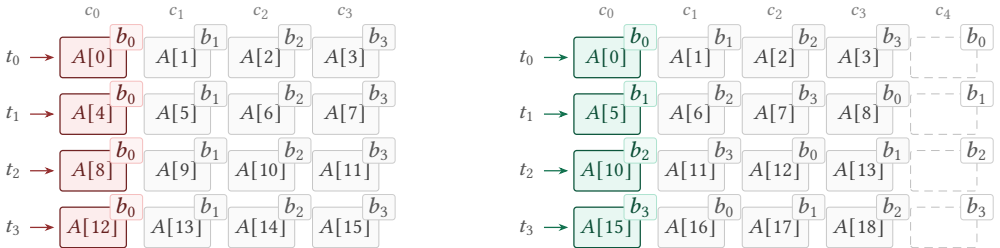
Fig. 8. Bank conflicts occur when threads access data in the same memory bank. In this example, we consider a 4 \times 4 tile of a matrix, stored in A , and use a warp size of four threads for simplicity. On the left, naively filling A with the tile’s entries causes values in the same column to be stored in the same bank, so threads accessing such values must serialize. On the right, adding a column of padding to A ensures that there is always one more element per row than threads per warp. Threads thus access different banks and can access SHMEM in parallel.
