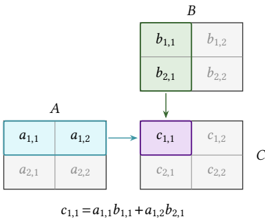
Fig. 10. Left: how rows and columns of the input matrices combine to produce the output matrix. Right: a naïve GEMM in CUDA. A simple matmul is a special case of GEMM where \alpha = 1 and \beta = 0 .
