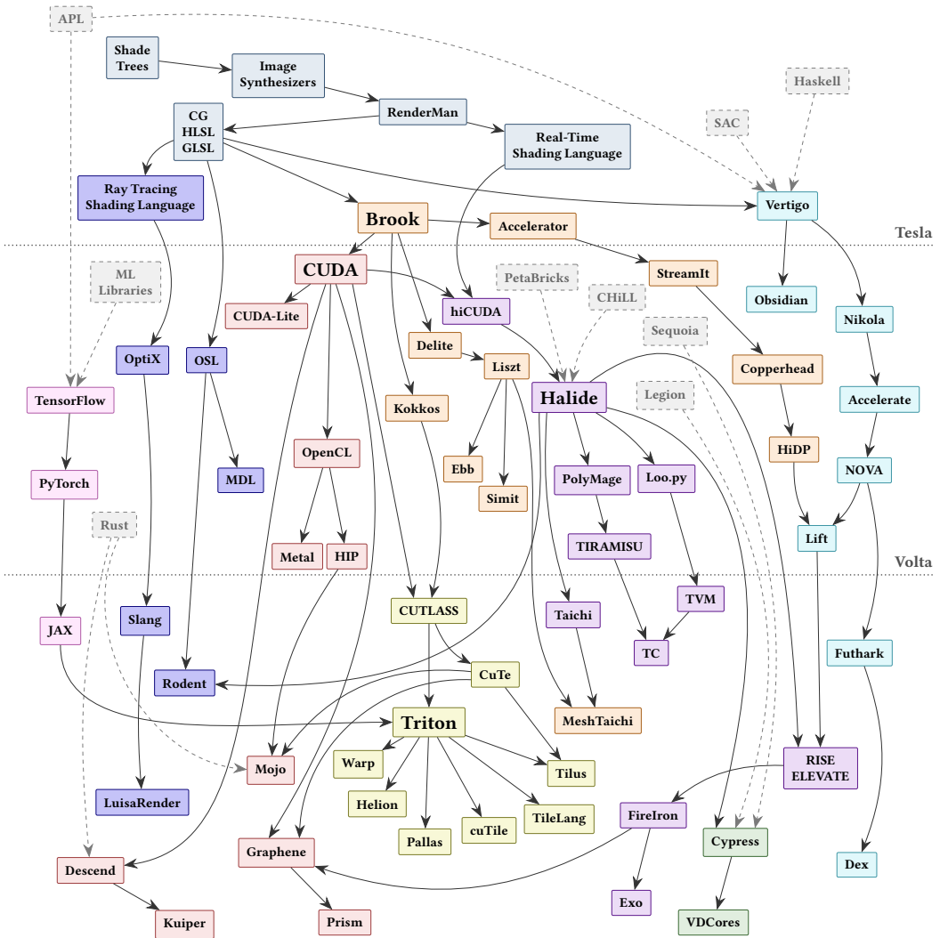
Fig. 16: A genealogy of GPU programming languages, connected by arrows when one inherits its ideas or goals from another. Languages sharing a color are discussed in the same subsection; dashed gray boxes indicate languages primarily used outside the GPU space. Languages are (roughly) temporally sorted, with the horizontal dotted lines indicating the release of major new architectures. In the rest of this section, we present several sub-genealogies, highlighting particular language families in more detail.
