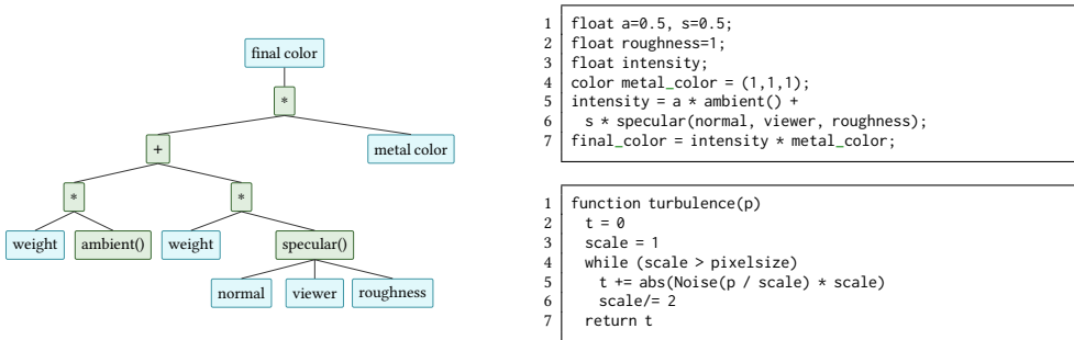
Fig. 17. Early graphics shading frameworks. Left: a shade tree, from Cook [83]. Top right: the shader program corresponding to the tree, also from Cook [83]. Bottom right: an image synthesizer, from Perlin [278].
