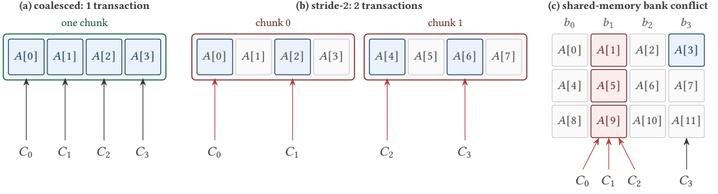
Fig. 3. Access patterns on a fictional GPU with 4 Cores per warp scheduler, 4-word chunks, and 4 shared-memory banks (real NVIDIA GPUs use 32 of each). In (a), consecutive loads coalesce into one transaction; in (b), loads touch two chunks and fetch twice the data they need; in (c), word A[i] lives in bank (b_i \bmod 4) , so Cores C_0 , C_1 , and C_2 , which access A[1] , A[5] , and A[9] , serialize on bank 1 while C_3 reads A[3] in parallel.
