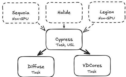
Fig. 33. Task-based languages for GPU programming.
