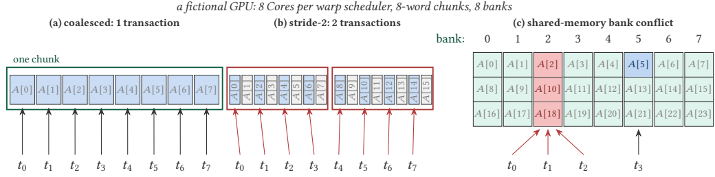
Fig. 3. Access patterns on a fictional GPU with 8 Cores per warp scheduler, 8-word chunks, and 8 shared-memory banks (real GPUs use 32 of each). (a) Consecutive loads coalesce into one transaction; (b) stride-2 loads touch two chunks and fetch twice the data they need. (c) Word A[i] lives in bank i \bmod 8 , so t_0 , t_1 , and t_2 , which access A[2] , A[10] , and A[18] , serialize on bank 2 while t_3 reads A[5] in parallel.
