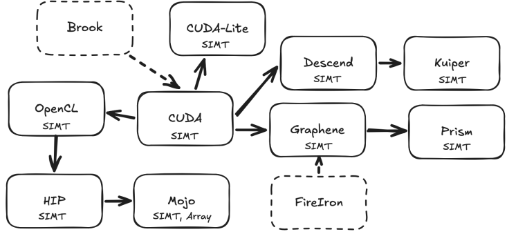
Fig. 16. GPU languages descended from CUDA [226].
