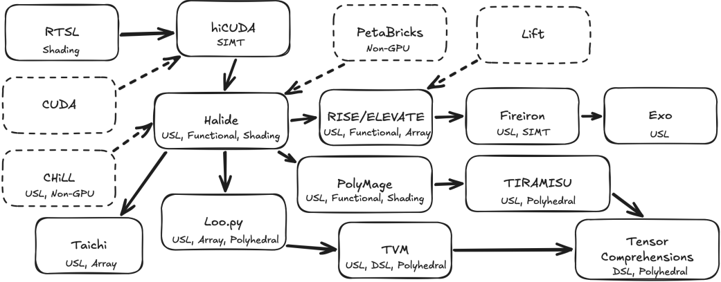
Fig. 23. GPU languages descended from Halide [277, 278].
