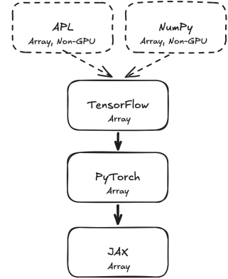
Fig. 22. Machine learning DSLs.
