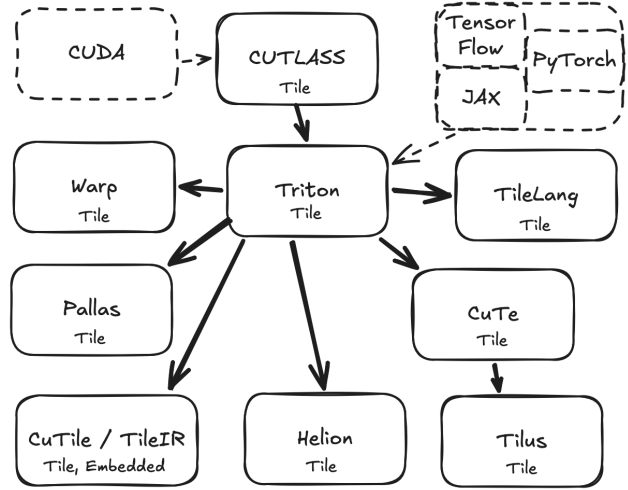
Fig. 29. GPU languages descended from Triton [331].
