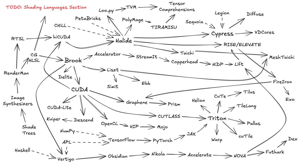
Fig. 10. A genealogy of programming languages for the GPU. Languages are connected by arrows when one inherits its ideas, theory, or implementation from another. Throughout the rest of this section we present a number of sub-genealogies, highlighting particular language families in more detail. [TODO: This figure is a work in progress: we are going to extend it to include the other languages discussed in Section 3.6 and reorganize it to be temporally sorted. However, feedback on any connections that are wrong or missing is very welcome.]
