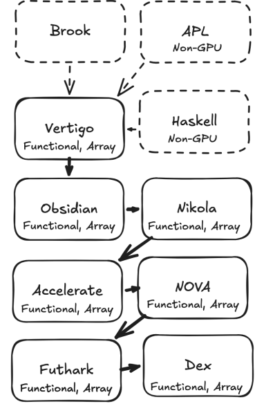
Fig. 19. Functional array languages for GPU programming.
