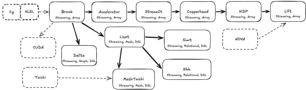
Fig. 12. GPU languages descended from Brook [46].
