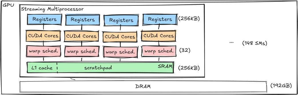
Fig. 2. Simplified SIMT hardware organization, annotated with approximate NVIDIA B200-scale capacities. Each SM contains four warp schedulers, groups of CUDA cores, a large register file, and SRAM partitioned between manually managed and automatically manager regions. SRAM is backed by whole-device. Concrete sizes given for a modern datacenter GPU (B200).
