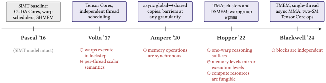
Fig. 9. Five generations of NVIDIA microarchitectures. Above the timeline, the major hardware capabilities each generation introduced; below, the SIMT assumptions that those capabilities removed (marked \ominus , in red).
