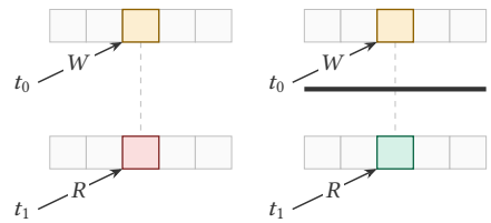
Fig. 46. GPUVerify [38]’s SDV semantics. Left: reading a pending write causes a run-time error. Right: after synchronizing, the read succeeds.
