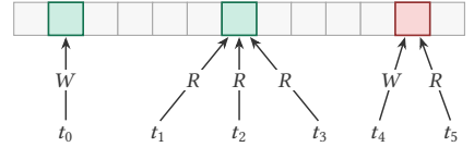
Fig. 47. VerCors [43] allows each memory location an exclusive writer or shared readers. A writer and reader at the same location conflict.
