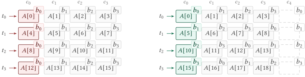
Fig. 8. Bank conflicts occur when threads access data in the same memory bank. In this example, we consider a 4 \times 4 tile of a matrix, stored in A , and use a warp size of four threads for simplicity. On the left, naively filling A with the tile’s entries causes values in the same column to be stored in the same bank, so threads accessing such values must serialize. On the right, adding a column of padding to A ensures that there is always one more element per row than threads per warp. Threads thus access different banks and can run in parallel.
