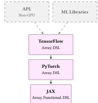
Fig. 29. Machine learning DSLs.
