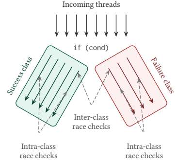
Fig. 45. Parametric flows handling a conditional in GKLEE p [207]. Races are checked between pairs of arbitrary threads within the classes that succeed and fail the conditional, and between representatives of the two classes.
