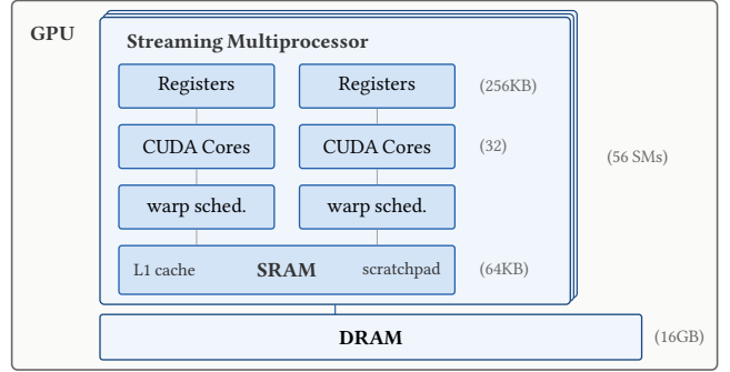
Fig. 2. Simplified SMT hardware organization, annotated with NVIDIA Pascal P100-scale capacities. A GPU contains many streaming multiprocessors (SMs); each SM has two warp schedulers, two groups of CUDA Cores, a large partitioned register file, an L1 cache (SRAM), and programmer-managed shared memory (scratchpad). All SMs share the GPU’s off-chip DRAM.
