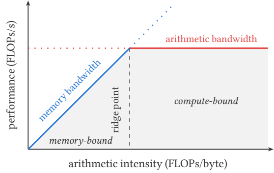
Fig. 5. The roofline model [363]. A kernel's maximum attainable performance is capped by the lower of two ceilings; kernels to the left of the ridge point are memory-bound, while those to its right are compute-bound.
