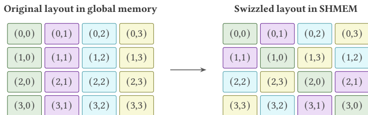
Fig. 13. A swizzle of a 4 \times 4 tile. Labels (r,c) identify the original location of elements. The swizzle moves each entry to column c \oplus r without changing its row, where \oplus is bitwise XOR.
