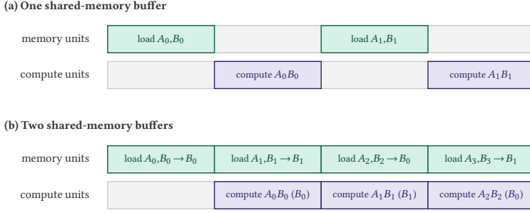
Fig. 13. Top: one shared-memory buffer means that either memory units or compute units are idle. Bottom: double buffering ensures that the hardware is always busy. B_0 indicates buffer 0; B_1 is buffer 1.
