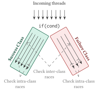
Fig. 42. Parametric flows handling an if statement. Races are checked between pairs of arbitrary threads within the classes of threads that succeed and fail the conditional check and between representatives of the two classes.
