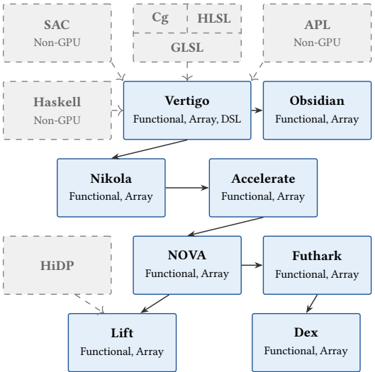
Fig. 25. Functional array languages for GPUs.
