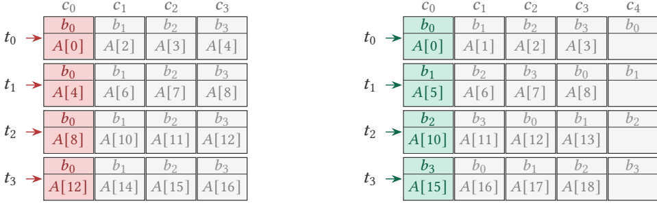
Fig. 9. A bank conflict occurs when multiple threads access data in the same memory bank. In this example, we consider a 4 \times 4 tile of a matrix, stored in array A; we use a warp of four threads, as opposed to the standard 32, for simplicity. On the left, naively filling A with the tile's entries causes values in the same column to be stored in the same bank, so threads accessing such values must run serially. On the right, adding an extra column of padding to A ensures that there is always one more element of each row than there are threads in a warp. Threads thus access different banks and can run in parallel.
