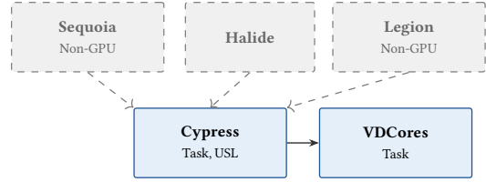
Fig. 39. Task-based languages for GPU programming. Cypress [357], which attempted to unify task-based programming with user-scheduling; programs comprise a logical specification and a mapping specification —essentially an algorithm-schedule distinction, except that Cypress’s mapping specifications assign tasks to different groupings of threads. The logical specification for a GEMM task, for example, is initially mapped to the entire grid; this mapping is then recursively decomposed into subtasks for blocks, warp-groups, warps, and eventually threads. Each level of the hierarchy has an associated mapping with its own particular properties; each mapping can specify how to move data between the levels of the hierarchy as the task is decomposed, for example, but the block-level mapping can also specify if and how to perform warp-specialization. Cypress’s logical specifications elide the tricky details of synchronization or inter-thread communication, allowing the programmer to focus purely on their kernel’s logic; these details are instead specified in the mapping specification and inserted by the compiler along with efficient data movement to maximize use of the GPU’s compute resources.
