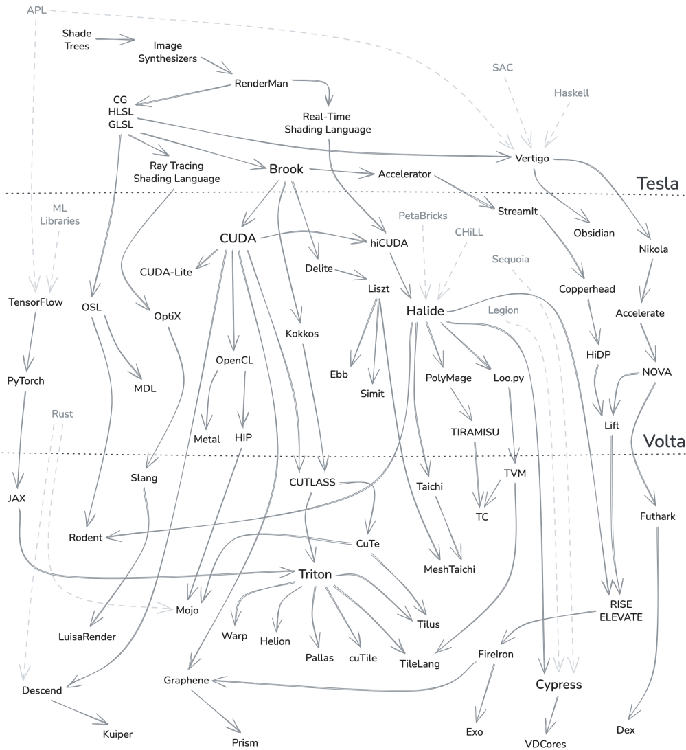
Fig. 16. A genealogy of programming languages for the GPU. Languages are connected by arrows when one inherits its ideas, theory, or implementation from another. Dashed arrows indicate connections from a language not originally designed for GPUs. The languages are (roughly) temporally sorted, with the horizontal dotted lines indicating the release of major new architecture designs. Throughout the rest of this section we present a number of sub-genealogies, highlighting particular language families in more detail.
