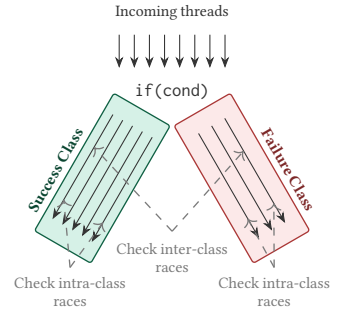
Fig. 43. Parametric flows handling an if statement. Races are checked between pairs of arbitrary threads within the classes of threads that succeed and fail the conditional check and between representatives of the two classes.
