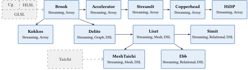
Fig. 19. Descendants of Brook [48]. Dashed boxes and lines indicate connections to or from languages outside this immediate slice of the genealogy in Figure 16.
