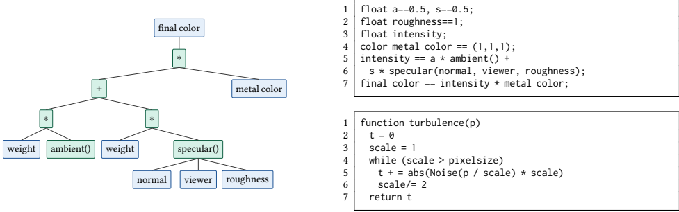
Fig. 17. Early graphics shading frameworks. Left: a shade tree, from Cook [78]. Top right: the shader program corresponding to the tree, also from Cook [78]. Bottom right: an image synthesizer, from Perlin [270].
