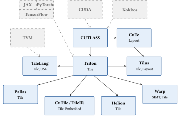
Fig. 36. Descendants of CUTLASS [325] and Triton [334].
