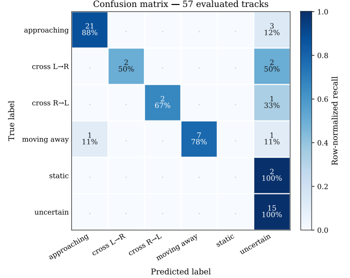
Figure 2: Confusion matrix on the 57 evaluated tracks. Off-diagonal errors are dominated by abstention into the uncertain column. The safety-critical approaching ↔ moving_away confusion is zero ; the only dangerous off-diagonal is one moving_away → approaching on a monotone bbox-growth edge case (IMG_4973/person_4).
