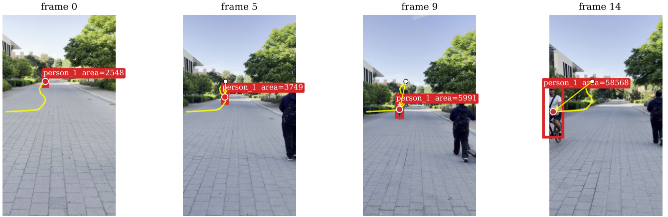
Figure 6: Temporal motion evidence for an approaching cyclist (IMG_4972/person_1, 15 frames). Area A = 2548 \rightarrow 58568 \text{ px}^2 , r = +21.98 ; centroid trail moves toward the lower centre; ego-motion-compensated flow is consistent with object motion rather than camera pan.
