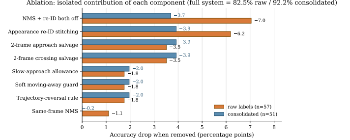
Figure 3: Accuracy drop when each component is removed (one at a time) from the full system. Tracker-side cleanups dominate; ByteTrack underperforms on sparse low-fps footage. Full numerics in Section C.
