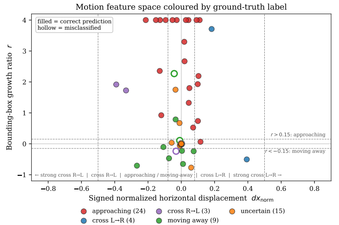
Figure 5: Motion feature space. Filled = correct, hollow = misclassified. Dashed lines are classifier thresholds. Growth values clipped to [-1.2, 4.0] for readability.
