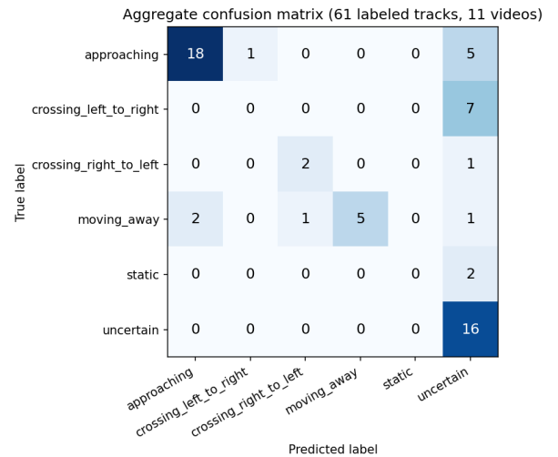
Figure 1: Aggregate confusion matrix across 11 videos / 61 labeled tracks (rows = ground truth, columns = predicted). The approaching column is clean (precision 0.90). The dominant error mode is uncertain false-negatives on the crossing_left_to_right row—driven by 1–2 frame tracker fragments where the classifier correctly abstains via the short_track rule.
