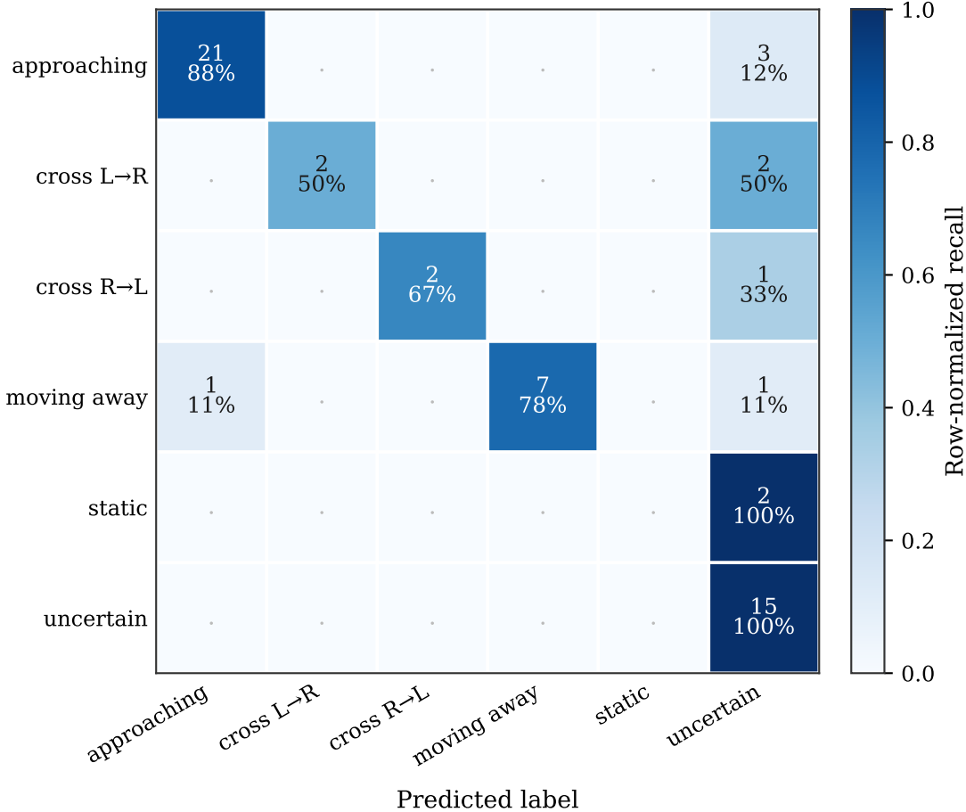
Confusion matrix — 57 evaluated tracks
