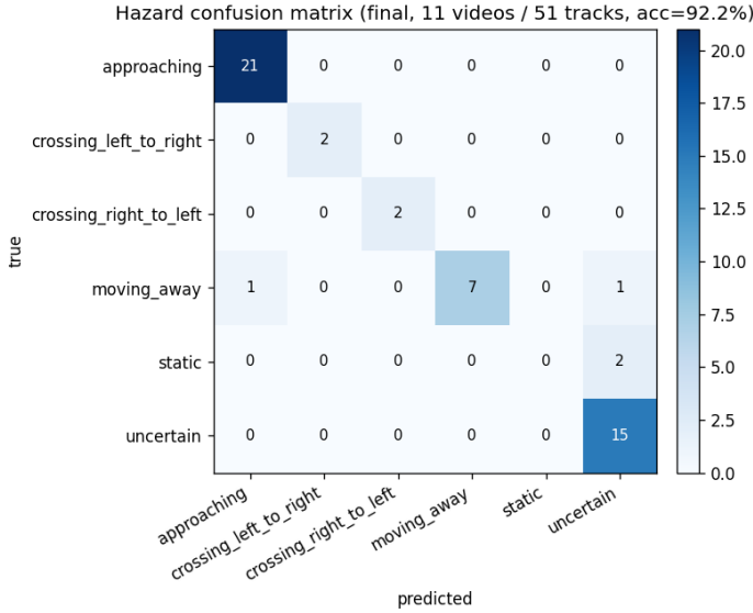
Figure 2: Final confusion matrix on consolidated labels (51 tracks). Rows: truth. Cols: prediction. The approaching column is precision-1.00 except for one moving_away → approaching (Fig. 3b).
