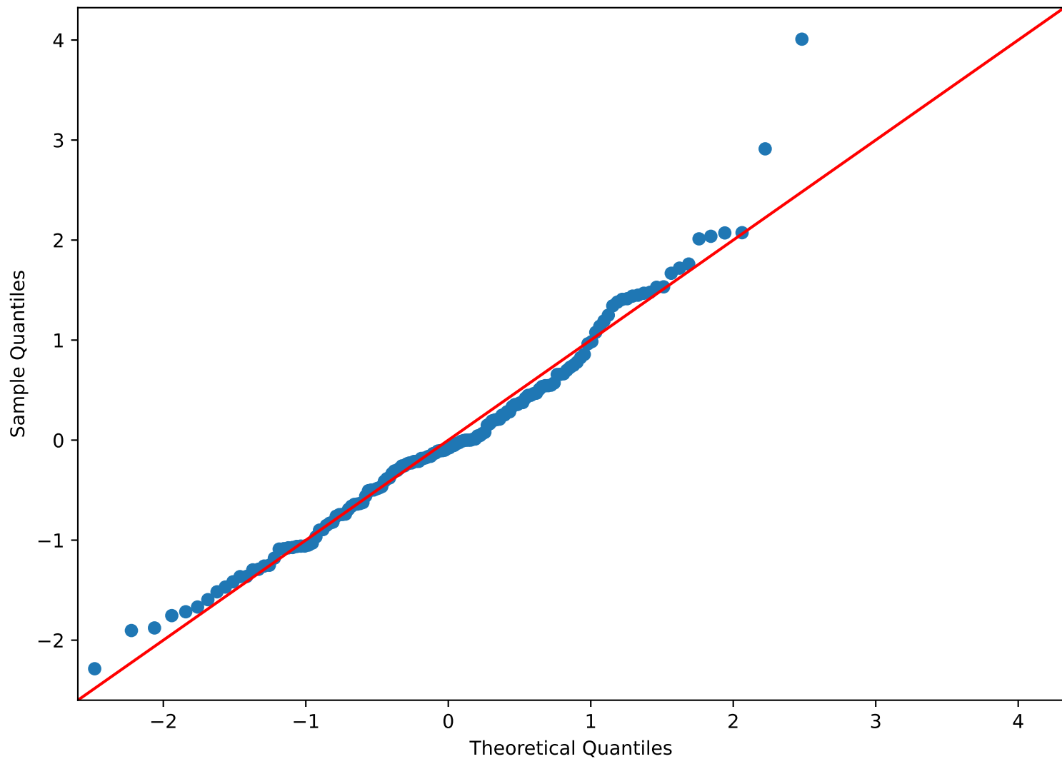
Normal Q-Q Plot of Standardized Residuals
