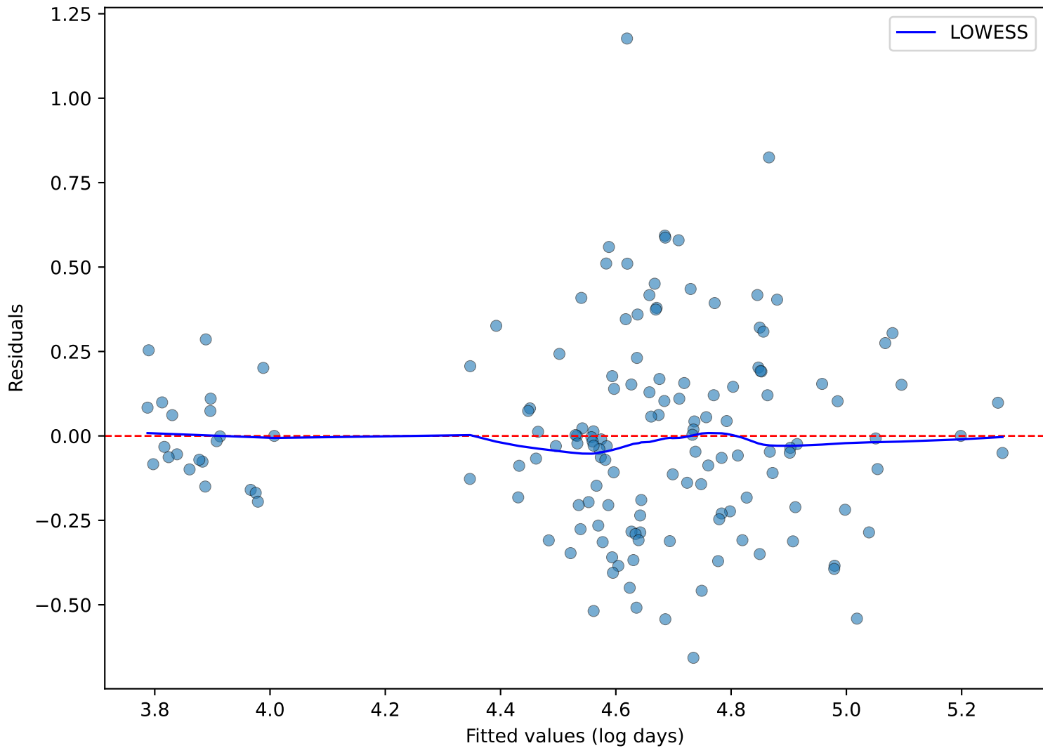
Residuals vs Fitted Values
