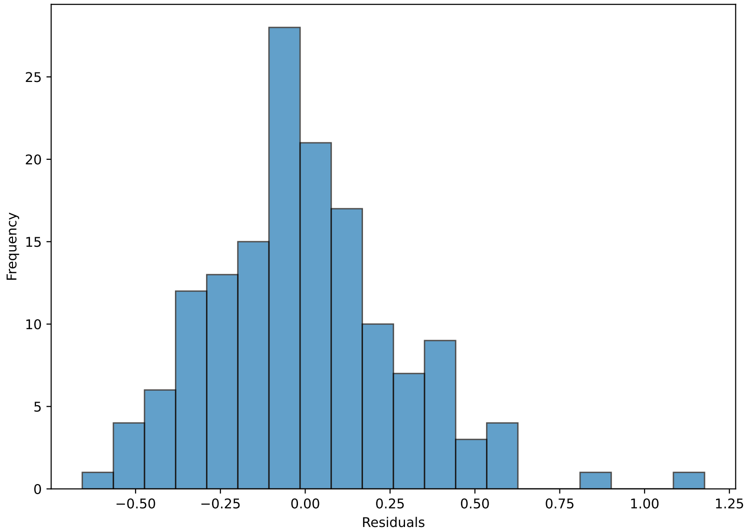
Distribution of Residuals
