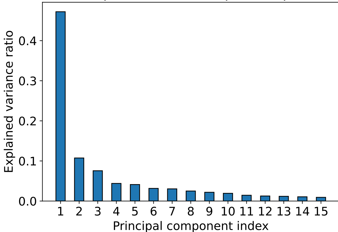
PCA: explained variance per component
