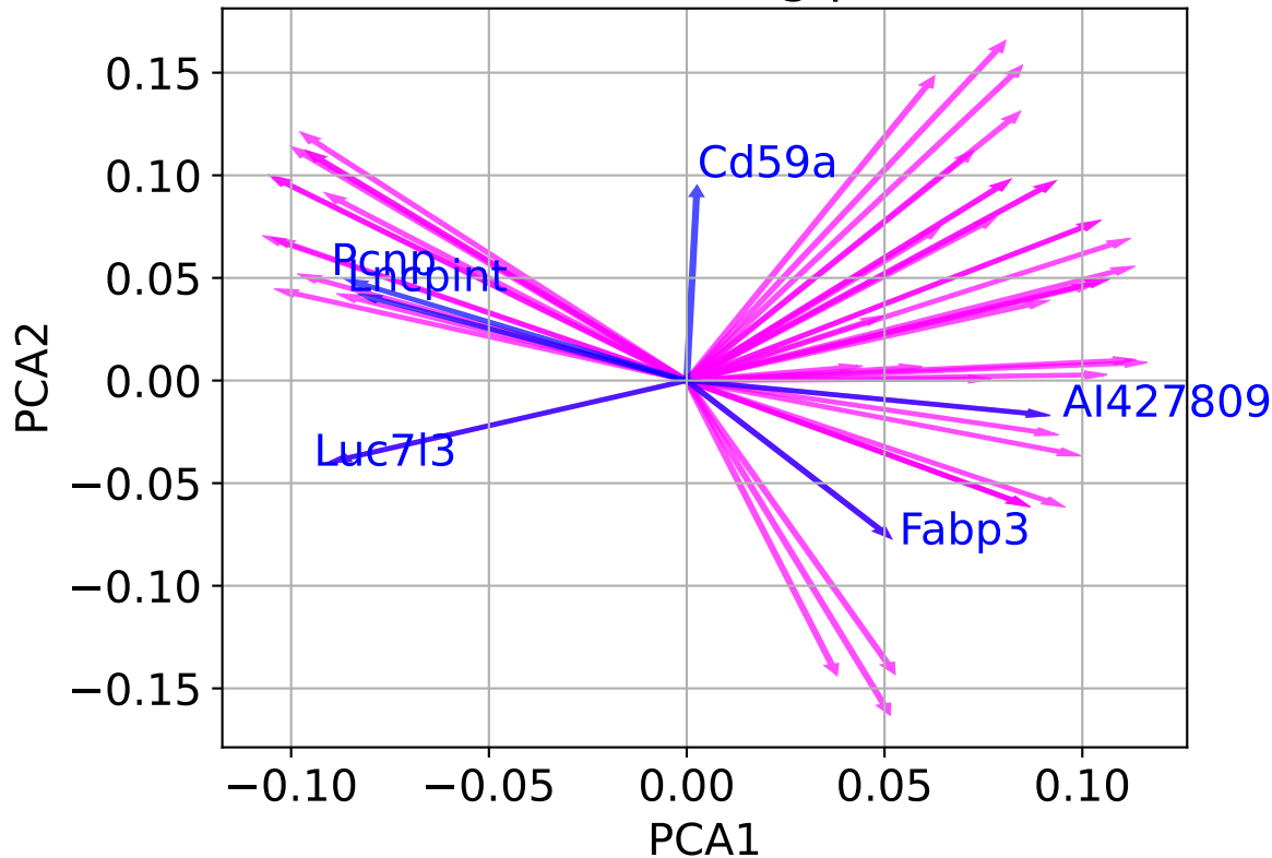
PCA: loading plot
