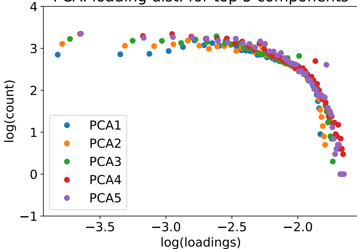
PCA: loading dist. for top 5 components
