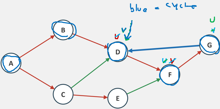
Blue back edge G to D closes D, F, G, D
