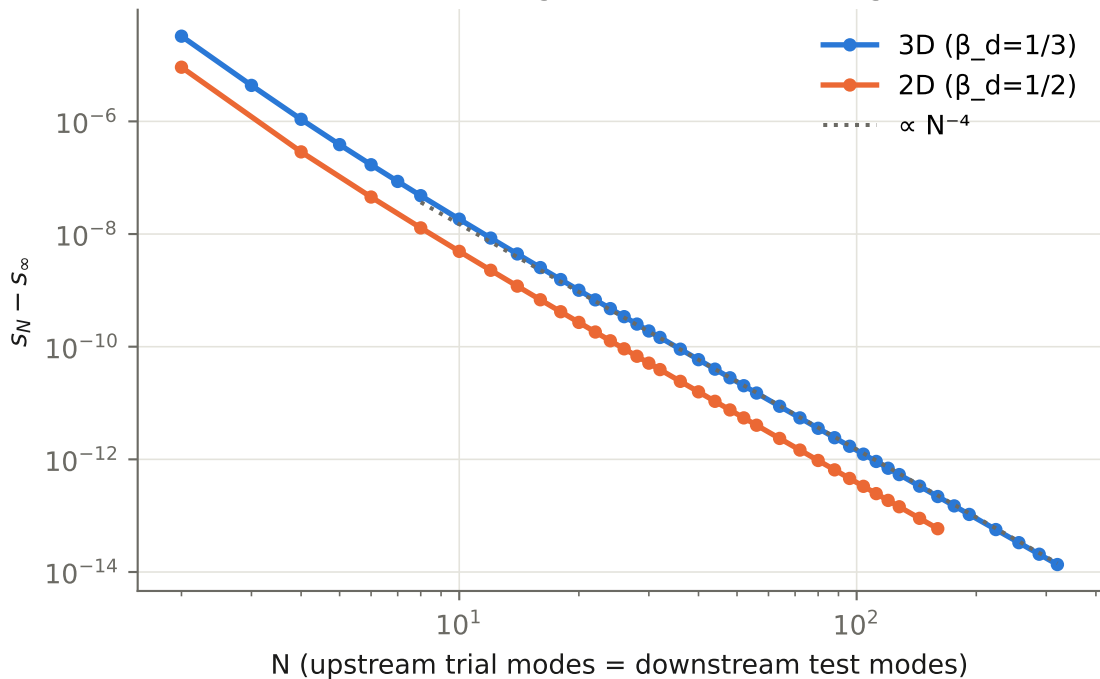
Truncation error of the eigenfunction matching
