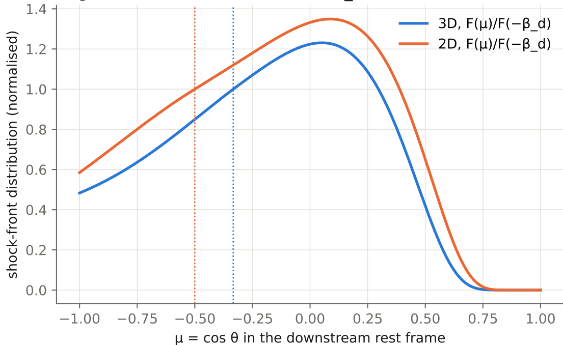
Angular distribution at the shock ( \Gamma_u \rightarrow \infty )
