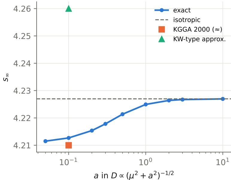
tangled-field scattering
