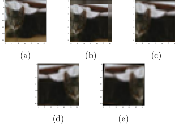
Figure 4: Augmentation pipeline
