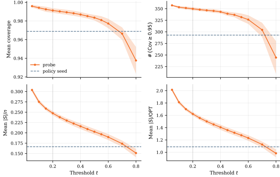
Figure 3: The probe’s coverage–cost operating curve over the threshold t , single pass, on the held-out test split (362 polygons). Top row is outcome, bottom row cost. Lines are the four-seed mean with \pm 1 std bands over probe seeds \{1234, 11, 22, 33\} ; the dashed line is the policy seed, which does not depend on t ; the dotted vertical marks the headline t = 0.20 . The two cost panels are the same curve at two scales — |S|/n and |S|/\text{OPT} are proportional to within 2.3% across the sweep — and are both shown so the cost can be read either as a fraction of vertices or as an approximation ratio. The bands widen with t , so the cheap end of the curve is also the less stable one.
