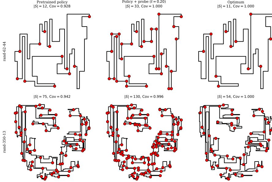
Figure 3: Two polygons drawn with the policy’s seed (left column), the policy plus the SETPREDICTOR probe at t = 0.20 (middle column), and the optimum (right column). Vertices selected as guards are marked. Row 1 is an in-distribution polygon where the policy already covers most of the region. Row 2 is an out-of-distribution polygon ( n = 350 , about 1.8\times the largest training polygon) where the policy’s seed falls below the 0.95 coverage gate ( \text{Cov}_P(\cdot) = 0.942 ) and the probe lifts it back above ( \text{Cov}_P(\cdot) = 0.996 ) at a guard cost typical for this split ( |S|/\text{OPT} \approx 2.4 ; cf. Table 8).
