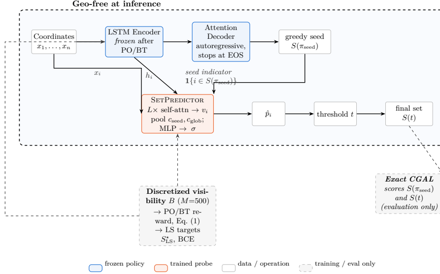
Figure 1: The full inference pipeline. The frozen LSTM encoder (trained by PO/BT, Section 4.1) turns vertex coordinates into per-vertex embeddings h_i ; its own decoder greedily decodes a seed guard set S(\pi_{\text{seed}}) . The SETPREDICTOR (Section 4.2) reads the frozen embeddings, the coordinates, and the seed indicator (Eq. (7)) and outputs a per-vertex probability \hat{p}_i , thresholded at t into the final guard set S(t) . Everything inside the dashed boundary is geo-free: no visibility object is read at the moment guards are placed (Section 2.3). Discretized visibility B (Eq. (4)) shapes the PO/BT reward and the SETPREDICTOR’s BCE targets S_{\text{LS}}^* during training only; exact CGAL scores both guard sets only at evaluation (Section 5.3) — both cross the geo-free boundary from outside it, never from within.
