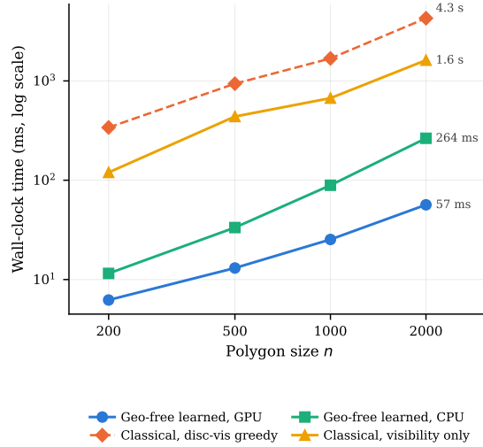
Figure 7: The runtime table as a growth curve (log-log; a constant vertical gap is a constant ratio). Geo-free inference (circles: GPU, squares: CPU) grows slowly with n ; classical visibility precompute (triangles) starts almost two orders of magnitude higher; disc-vis greedy (dashed diamonds) is higher still. Exact greedy is omitted here as a single anecdotal point (Table 11: \approx 13.8 s at n = 200 , unstable beyond it). Timing data of Table 11; the quality this speed costs is in Table 12.
