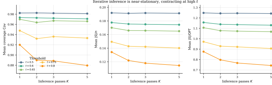
Figure 4: Iterative inference is near-stationary at the thresholds the probe is operated at, contracting slowly at the highest ones, on the held-out test split (362 polygons). Each panel shows mean coverage ( left ), |S|/n ( centre ), and |S|/OPT ( right ) versus inference passes K \in \{1, 2, 3, 5\} for thresholds t \in \{0.5, 0.6, 0.65, 0.75, 0.8\} — a higher range than the headline thresholds, where the property is most stringently tested near the decision boundary. Drift has a consistent direction — K = 5 sheds guards and loses a little coverage relative to K = 1 at every threshold — and grows with t : within noise at t = 0.5 , 0.079 in |S|/OPT at t = 0.8 (bounds in Section 6.5).
