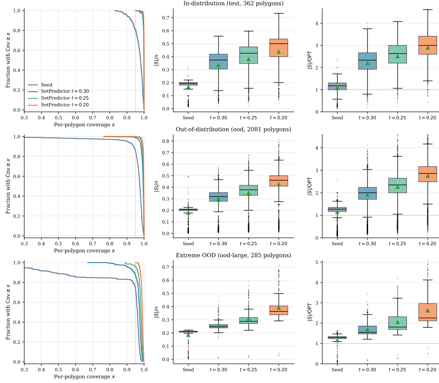
Figure 4: Distributional view of method performance across all three evaluation regimes: test (top, 362 polygons), ood (middle, 2081 polygons), and ood-large (bottom, 285 polygons, n up to 2250). Left : per-polygon coverage as a complementary stair-step CDF; the dashed line marks the 0.95 feasibility gate. Center, right : box plots of the normalized guard count |S|/n and the approximation ratio |S|/OPT for the policy seed and the three probe thresholds; for ood-large the |S|/OPT boxes cover only the 206/285 polygons with an available ILP solution and are therefore biased toward the smaller polygons of that split (which is why the tables report no approximation ratio on ood-large ; Section 5.3). Boxes show the displayed seed (1234); the four-seed mean \pm std is in Tables 3 and 6.
