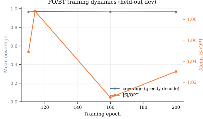
Figure 1: PO/BT training dynamics on the held-out dev split, reconstructed post-hoc from the four saved checkpoints — not a continuous online log;
