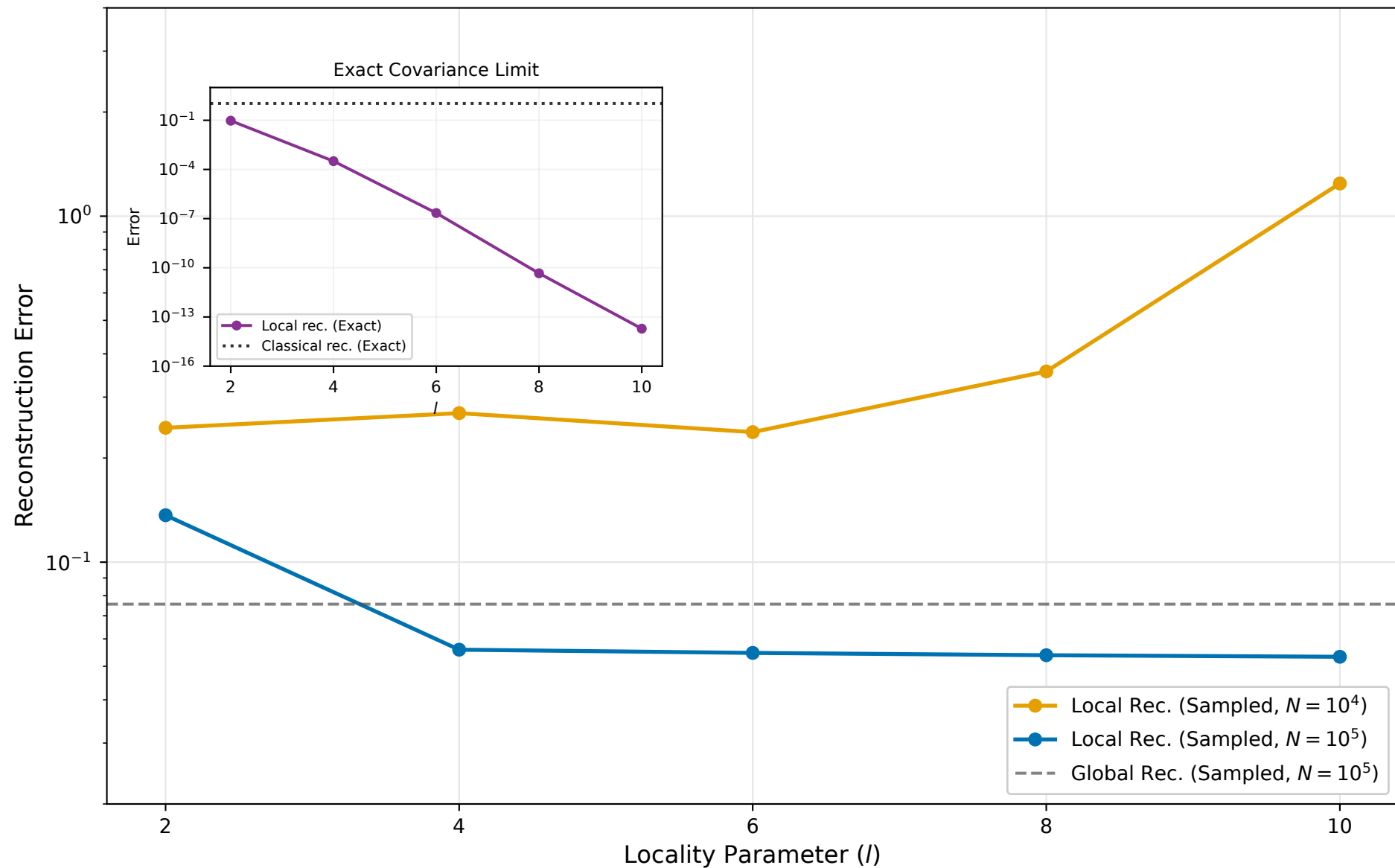
Convergence of Local Reconstruction vs Locality Parameter l (Fixed System Size m=100 )
