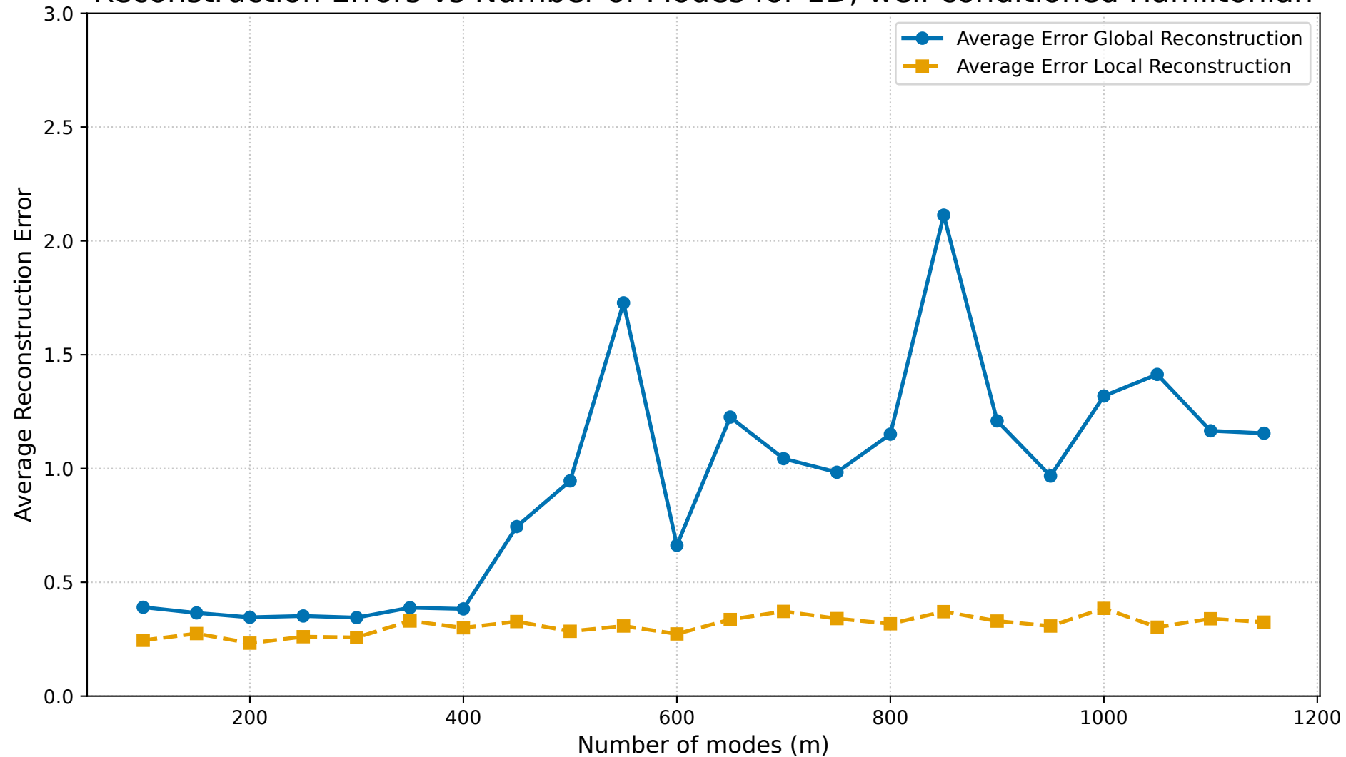
Reconstruction Errors vs Number of Modes for 1D, well-conditioned Hamiltonian
