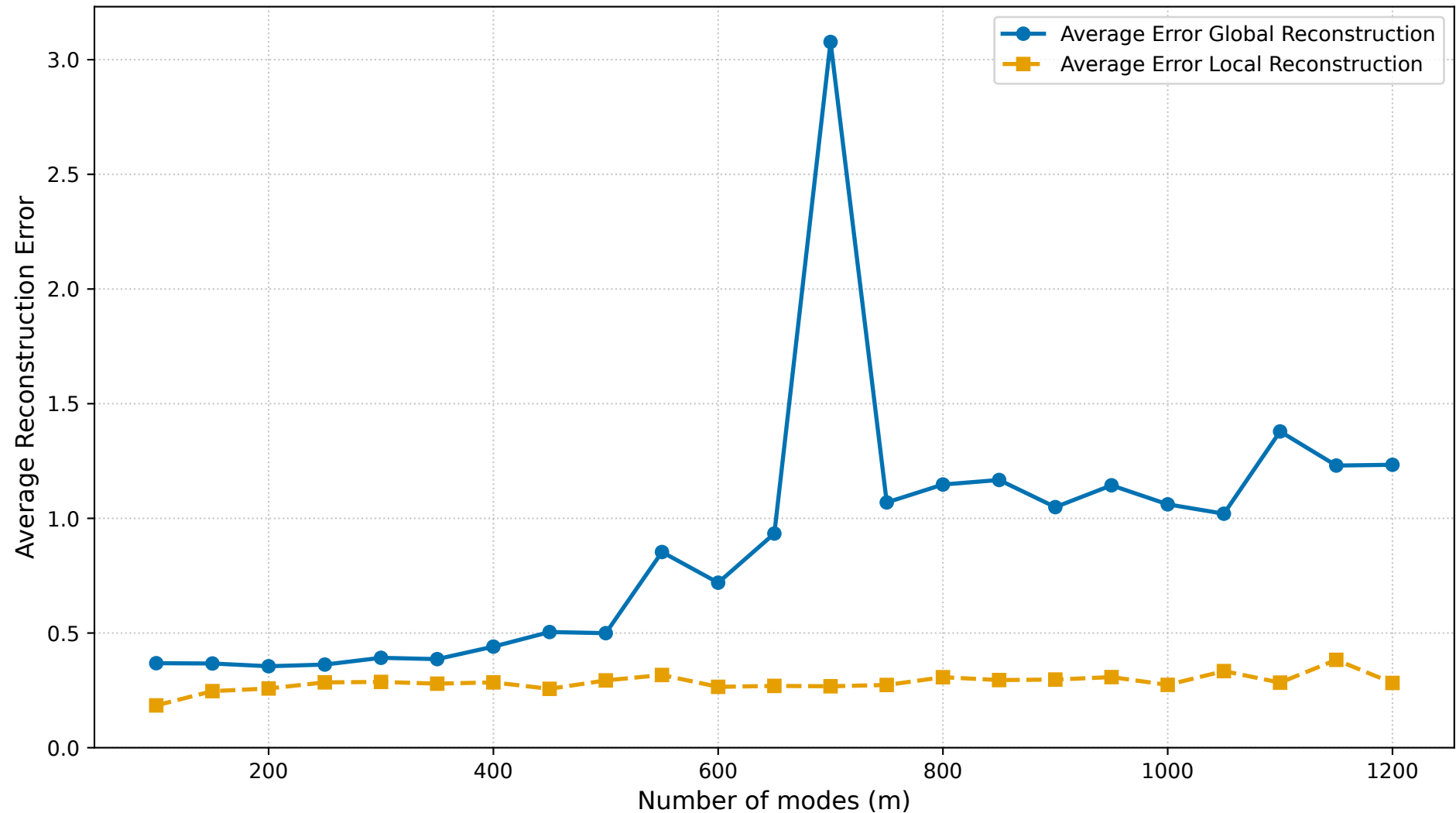
Reconstruction Errors vs Number of Modes for 1D, ill-conditioned Hamiltonian
