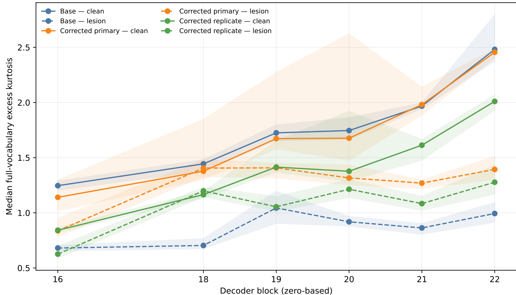
J-lens readout concentration: each model's own 500-prompt lens
