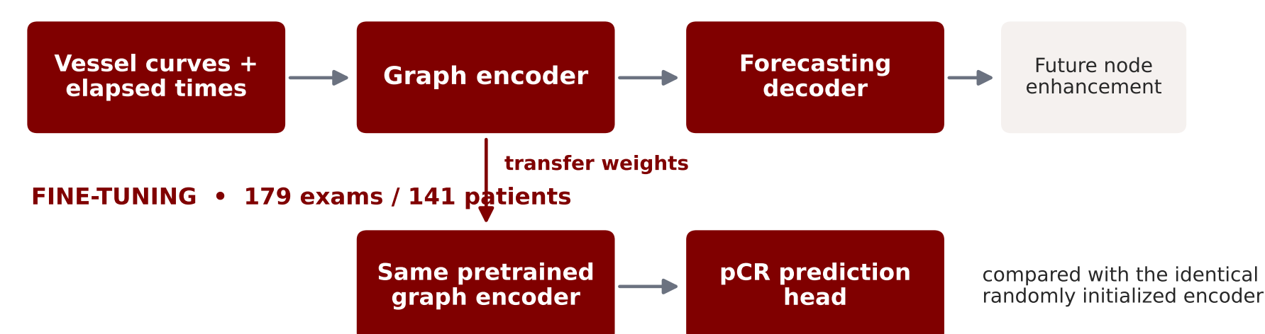
Figure 3. Forecasting weights initialize the downstream encoder.
