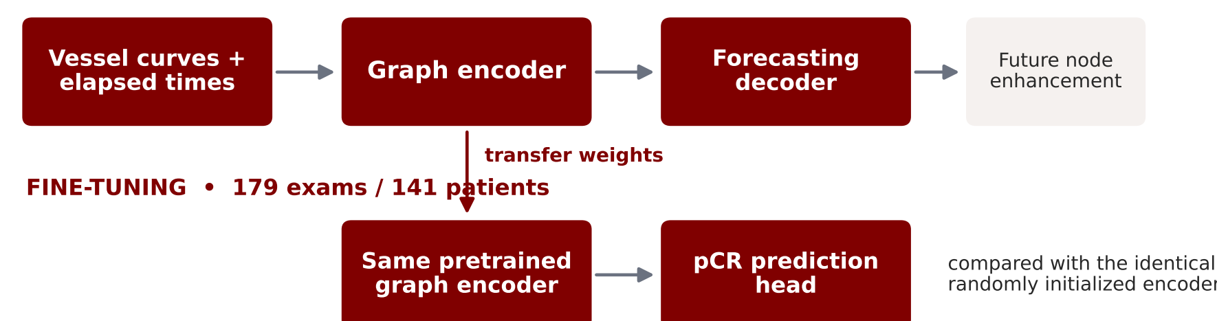
Figure 3. Forecasting weights initialize the downstream encoder.
