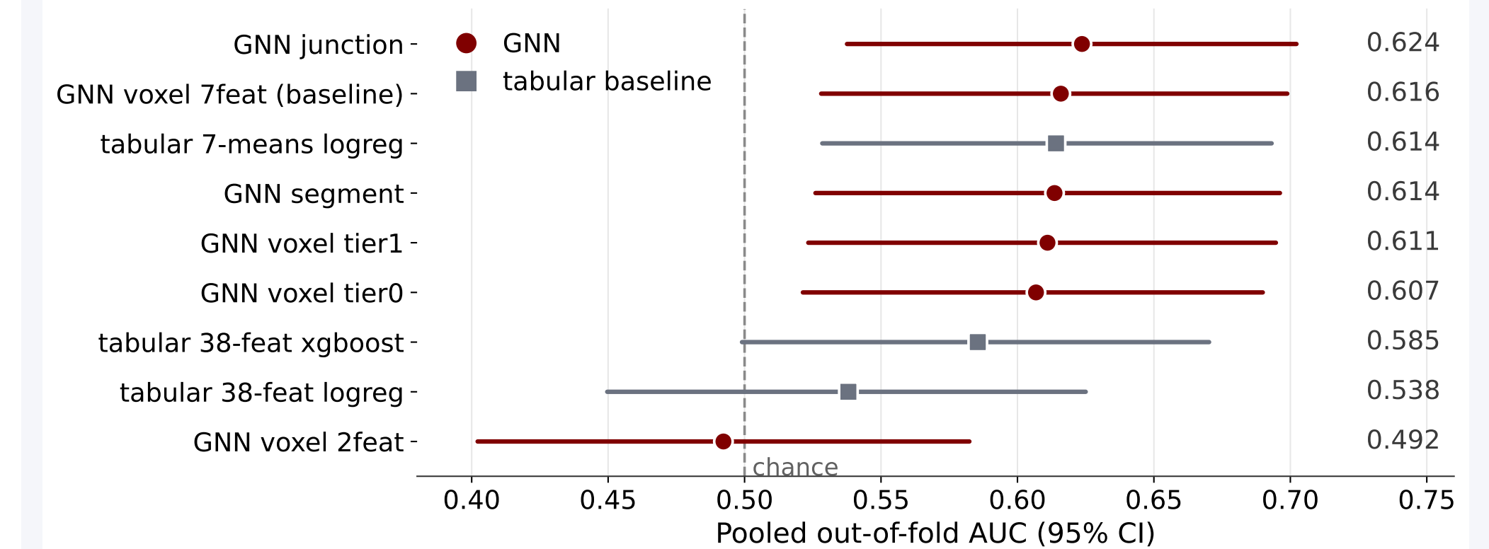
Figure 4. Pooled out-of-fold AUC, bootstrap 95% CI, shared folds. Preliminary.
