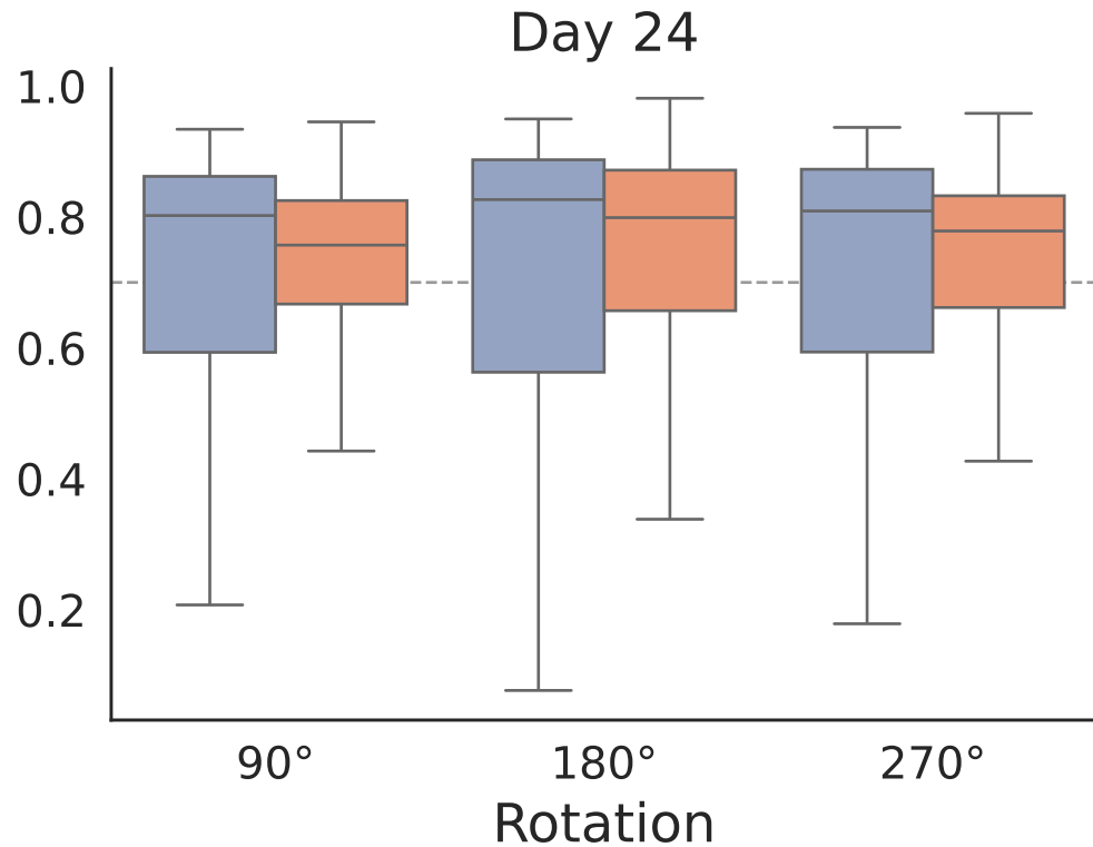
Grad-CAM rotation consistency (cosine)
