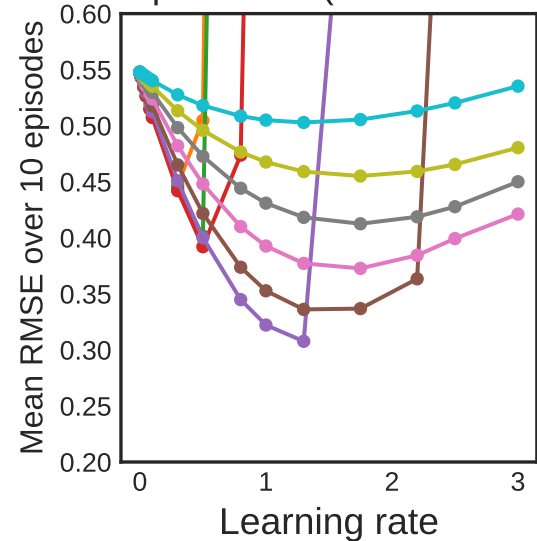
Emphatic TD (interest: 0.01)
