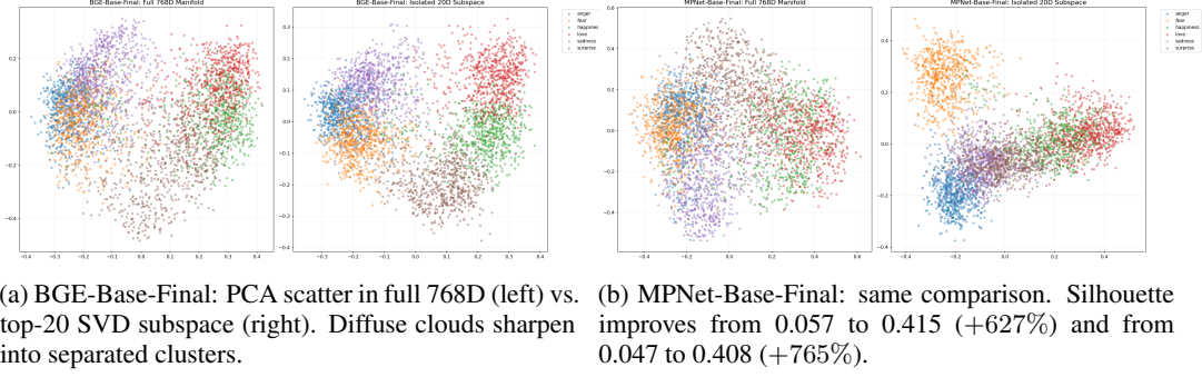
Figure 4: 768D vs. top-20 SVD subspace (Finding 3). Projecting into the 20-dimensional signal subspace reveals the cluster structure hidden by noise dimensions in the full embedding space.
