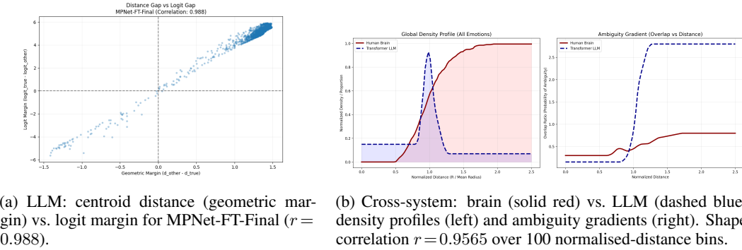
Figure 5: The cross-system ambiguity gradient. Both systems link geometric proximity to prototypes with representational certainty, through complementary mechanisms.
