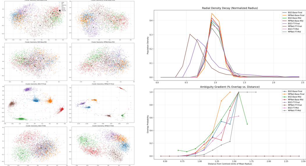
(a) PCA projections of all 8 LLM variants. Pre-trained models (rows 1–2): overlapping clouds with no visible cluster structure. Fine-tuned models (rows 3–4): compact, well-separated islands.
