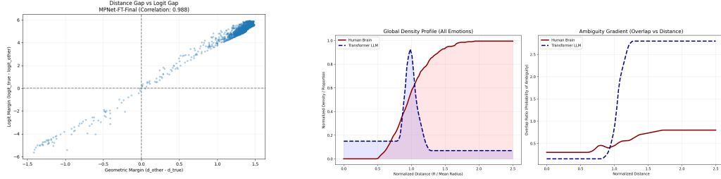
(a) LLM: centroid distance (geometric margin) vs. logit margin for MPNet-FT-Final ( r = 0.988 ). (b) Cross-system: brain (solid red) vs. LLM (dashed blue) density profiles (left) and ambiguity gradients (right). Shape correlation r = 0.9565 over 100 normalised-distance bins.
