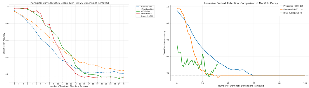
(a) Signal cliff: accuracy as dominant directions are removed iteratively. Fine-tuned models reach chance at dimensions 15–20; pretrained BGE at 26, pretrained MPNet at 67.
