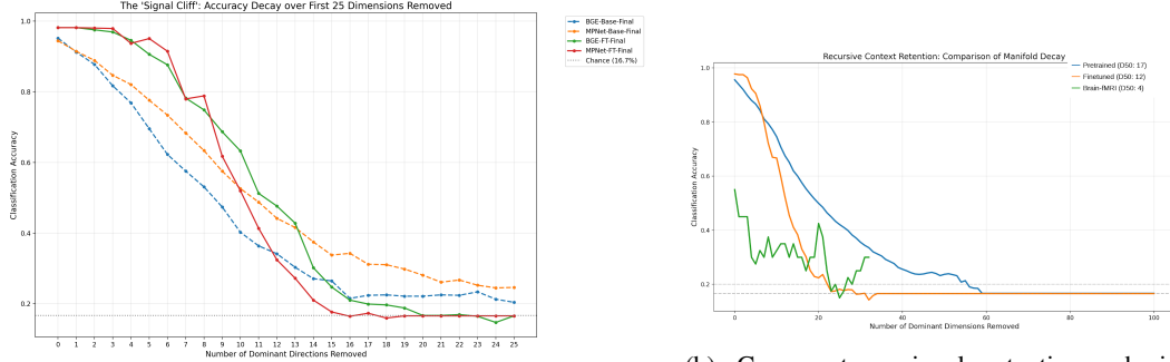
(b) Cross-system signal retention: brain ( D_{50} = 4 ), fine-tuned LLM ( D_{50} = 12 ), pre-trained LLM ( D_{50} = 17 ). The brain decays fastest initially but plateaus rather than collapsing.
